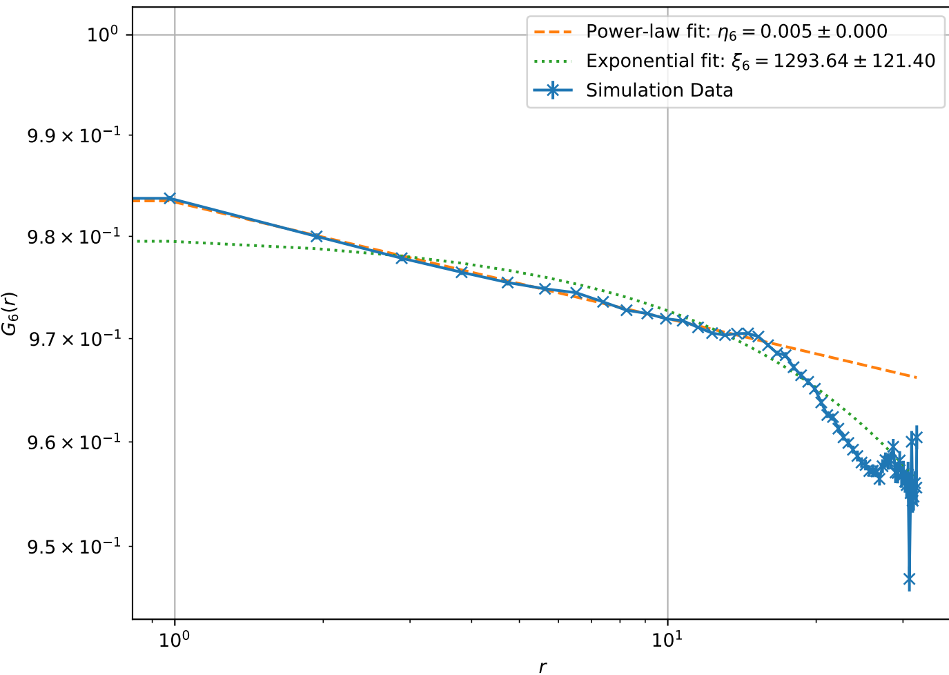
Correlation Function at T = 7.00e - 02 , L = 32 (Log-Log Scale)
