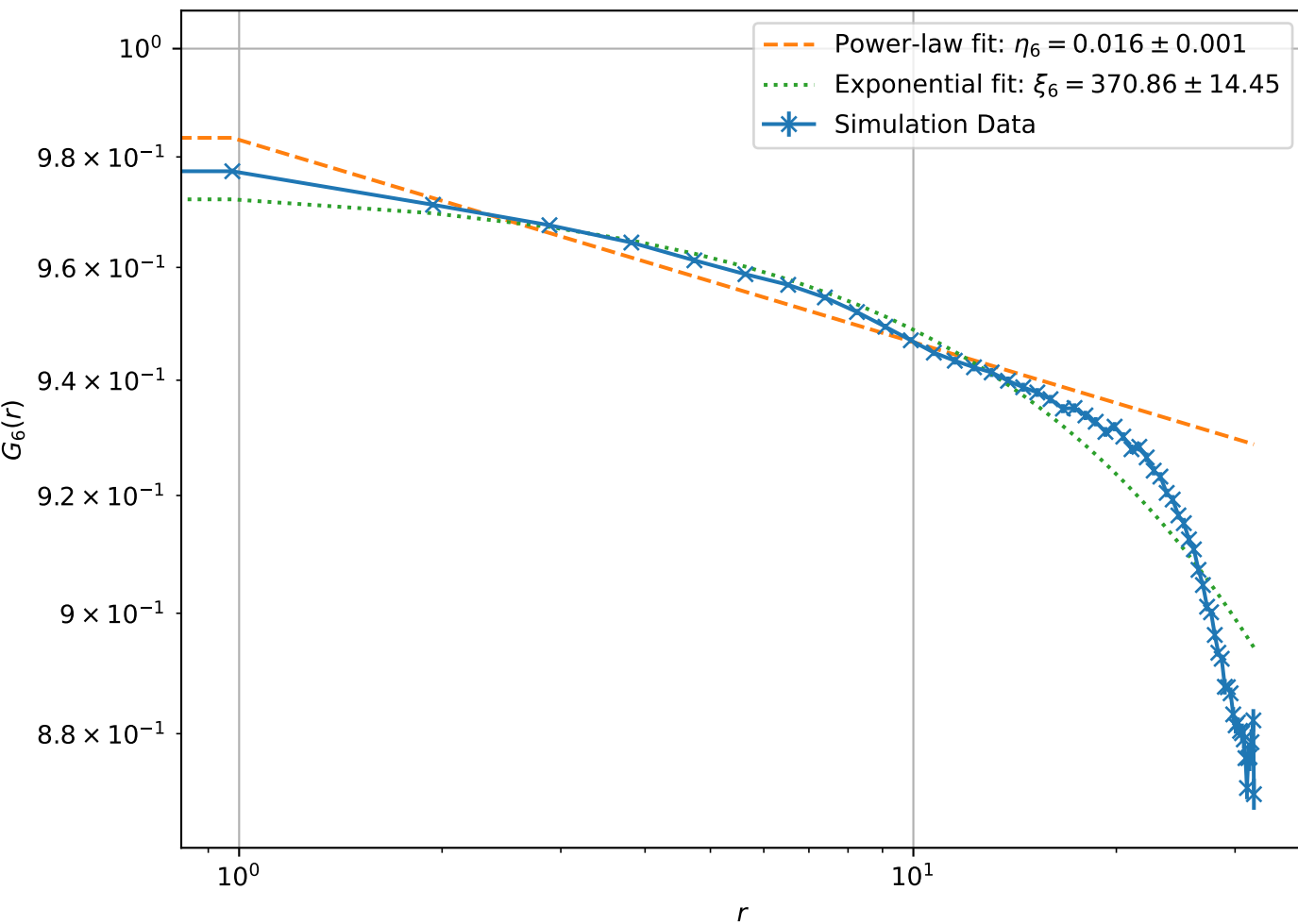
Correlation Function at T = 8.00e - 02 , L = 32 (Log-Log Scale)
