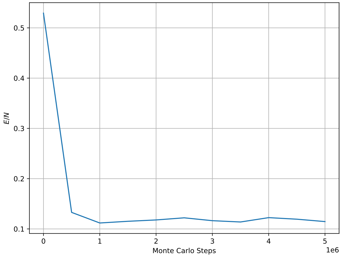
Energy per Spin at T = 9.00e - 02 , L = 32
