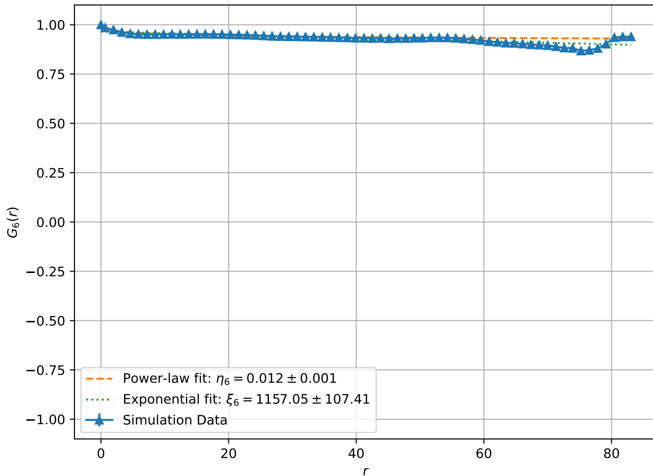
Correlation Function at T = 1.00e - 05 , L = 64
