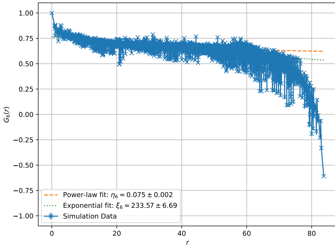
Correlation Function at T = 1.50e - 01 , L = 64
