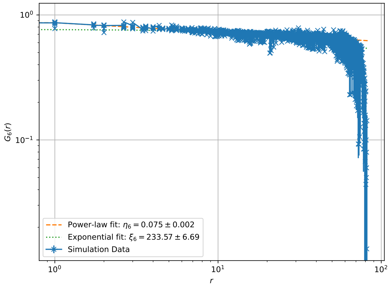
Correlation Function at T = 1.50e - 01 , L = 64 (Log-Log Scale)
