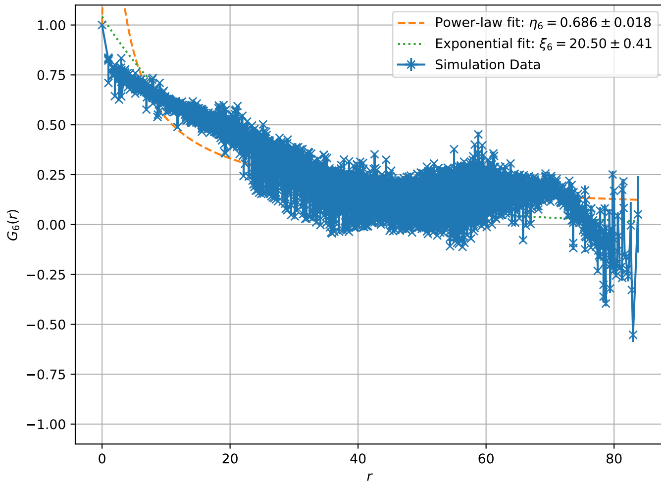
Correlation Function at T = 1.60e - 01 , L = 64
