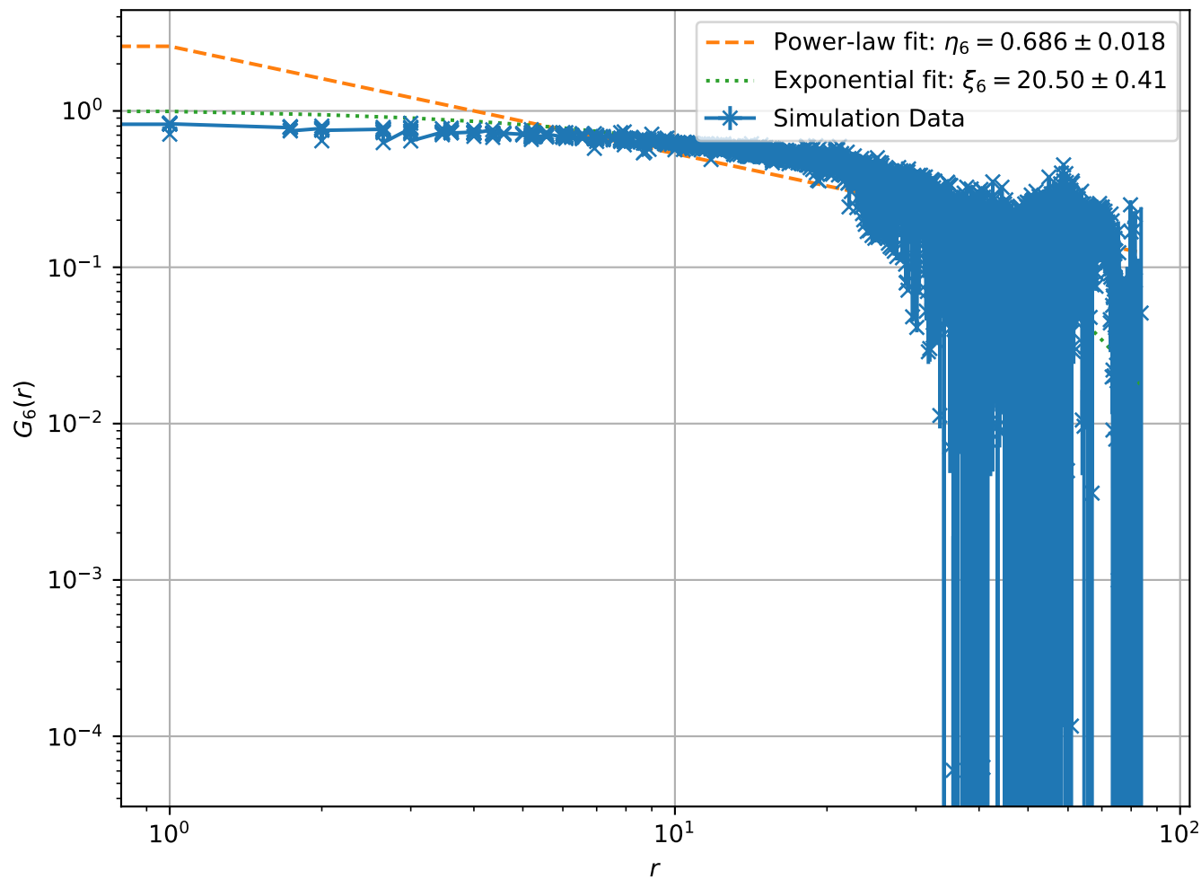
Correlation Function at T = 1.60e - 01 , L = 64 (Log-Log Scale)
