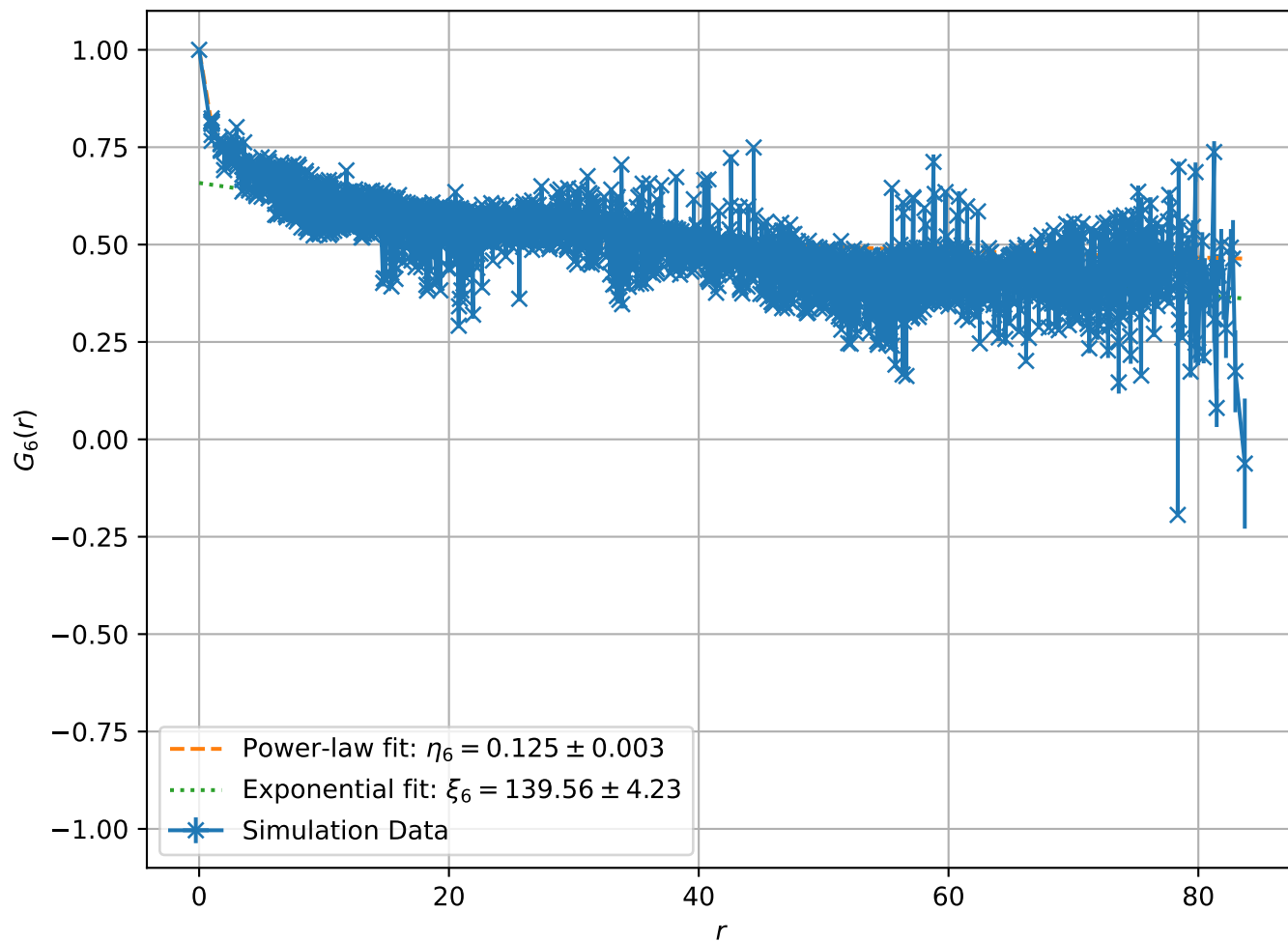
Correlation Function at T = 1.70e - 01 , L = 64
