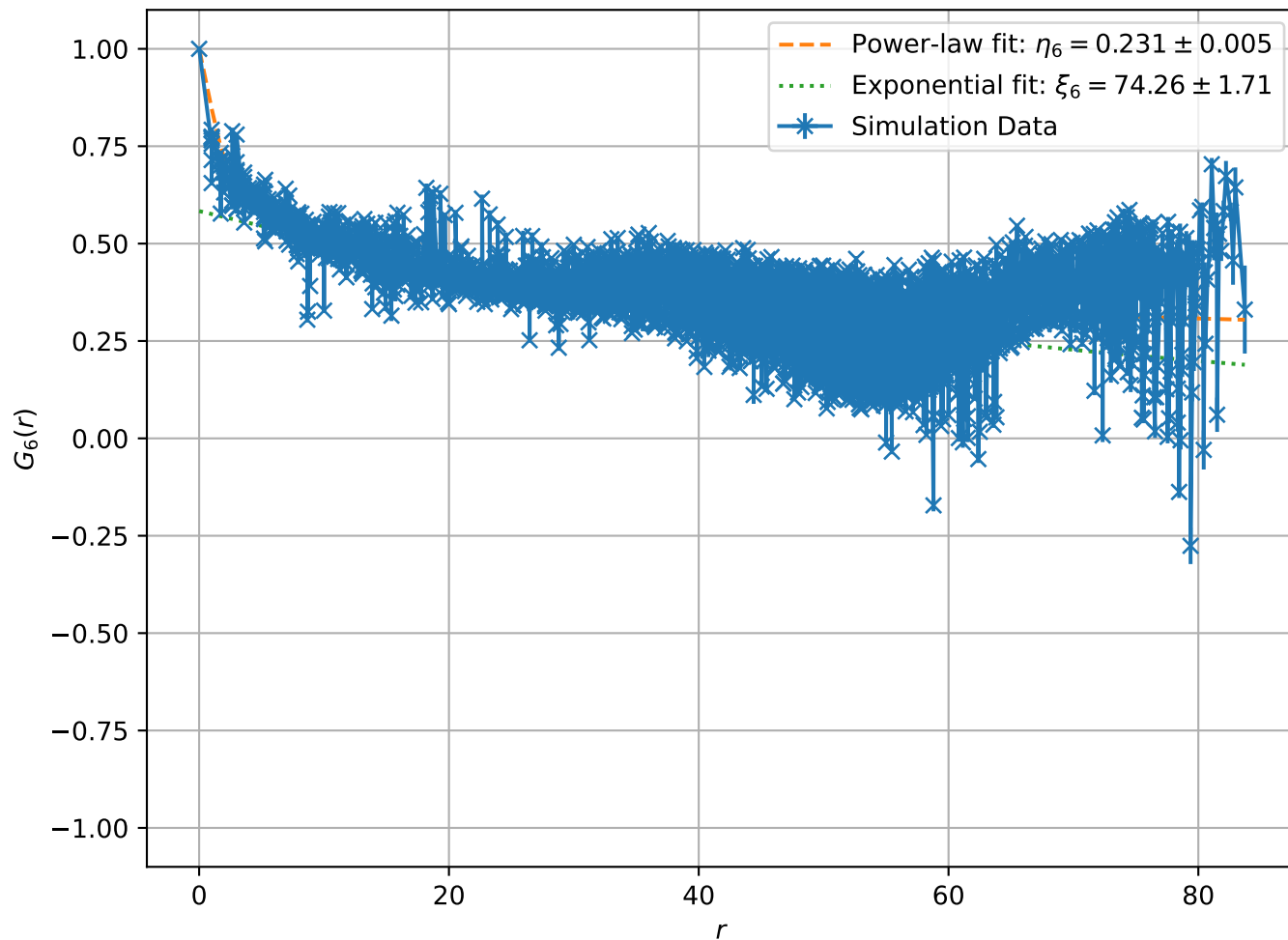
Correlation Function at T = 1.80e - 01 , L = 64
