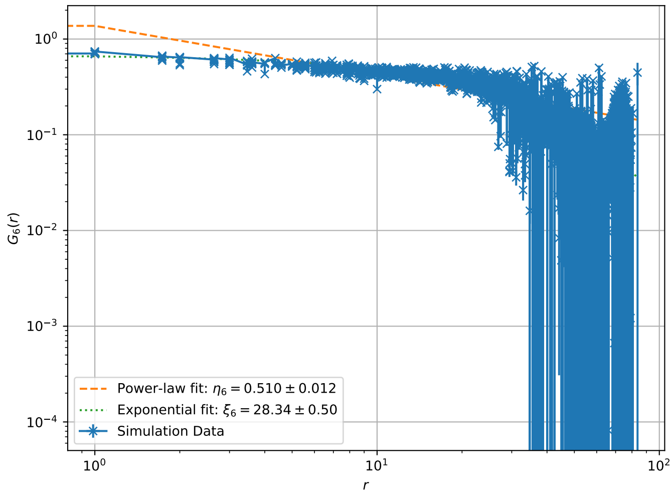
Correlation Function at T = 1.90e - 01 , L = 64 (Log-Log Scale)
