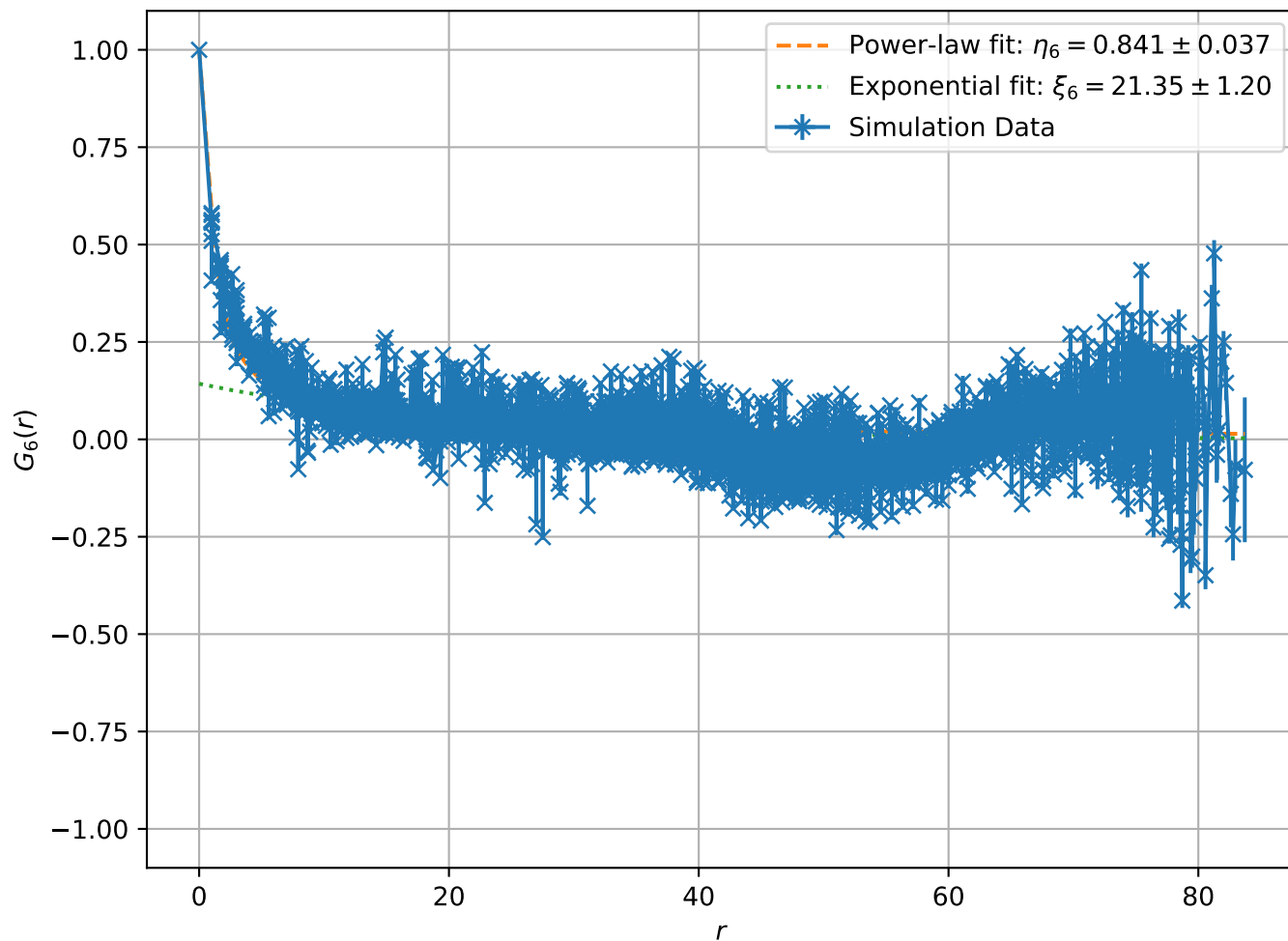
Correlation Function at T = 2.10e - 01 , L = 64
