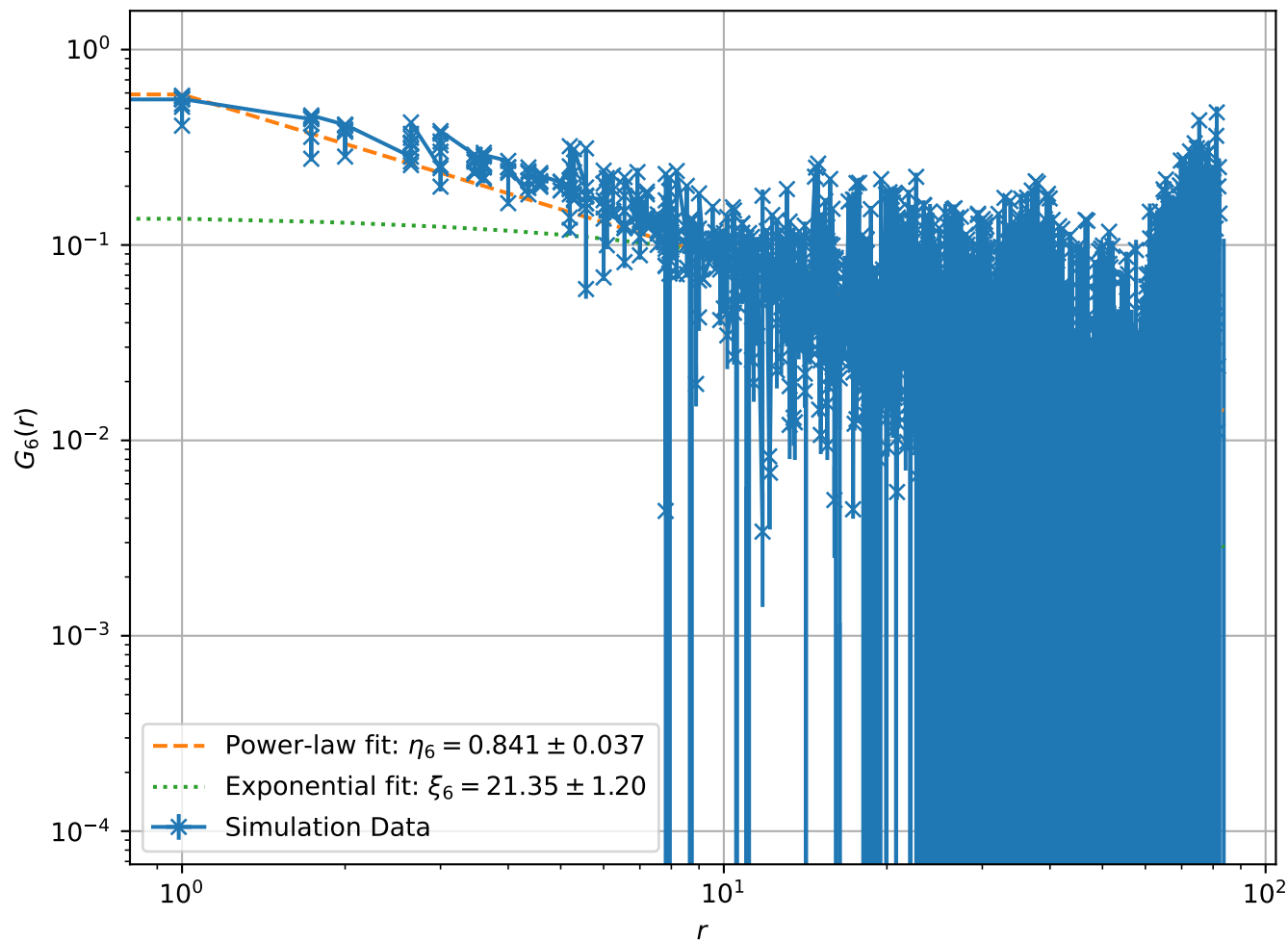
Correlation Function at T = 2.10e - 01 , L = 64 (Log-Log Scale)
