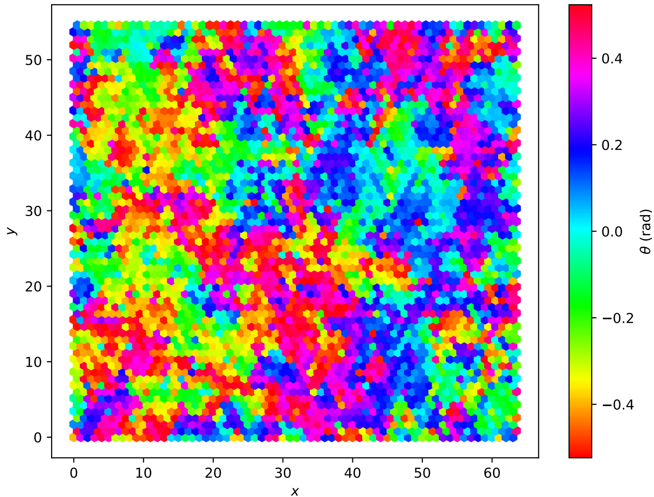
Hexagonal Lattice L=64 , T = 2.10e - 01
