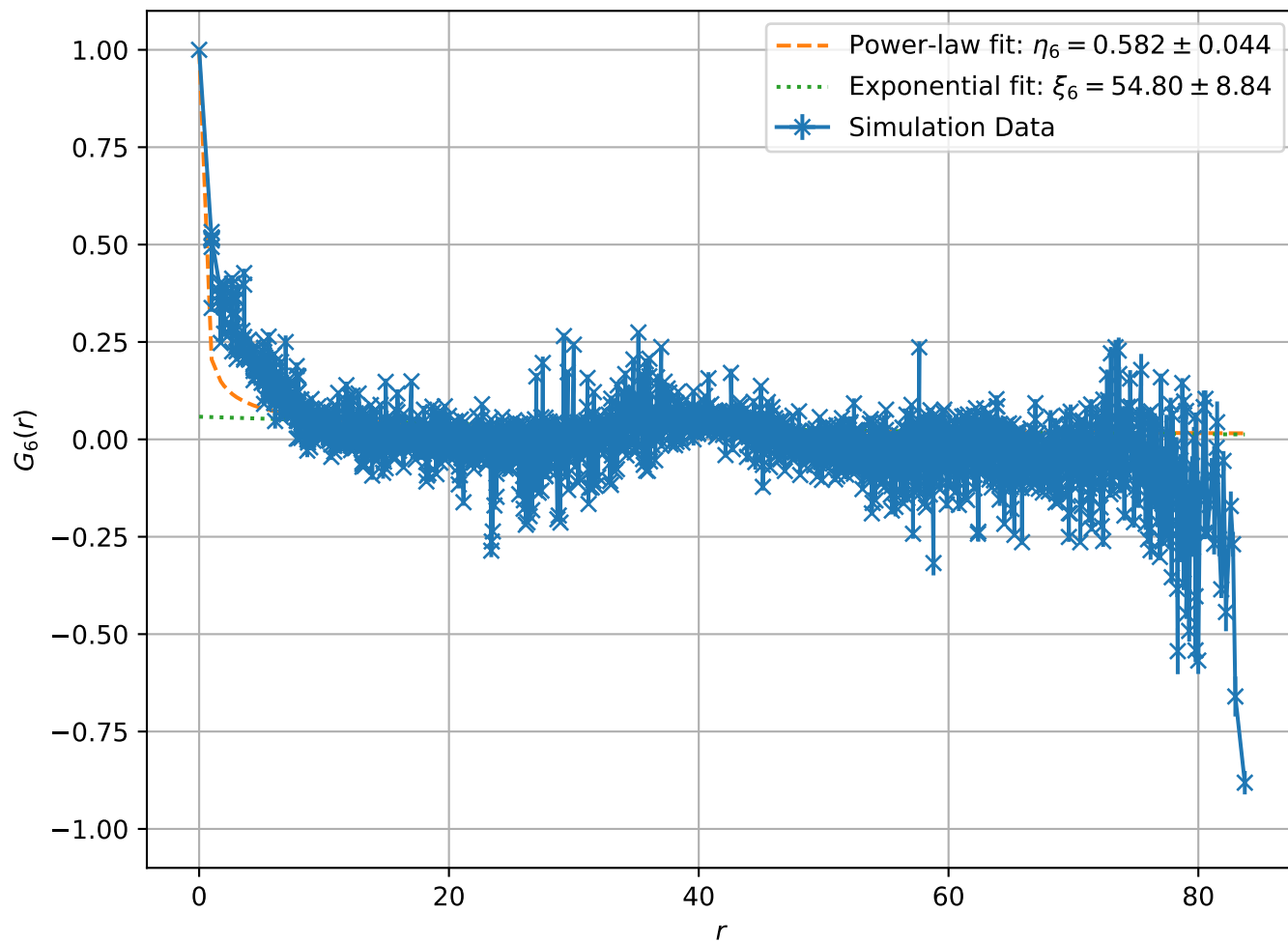
Correlation Function at T = 2.20e - 01 , L = 64
