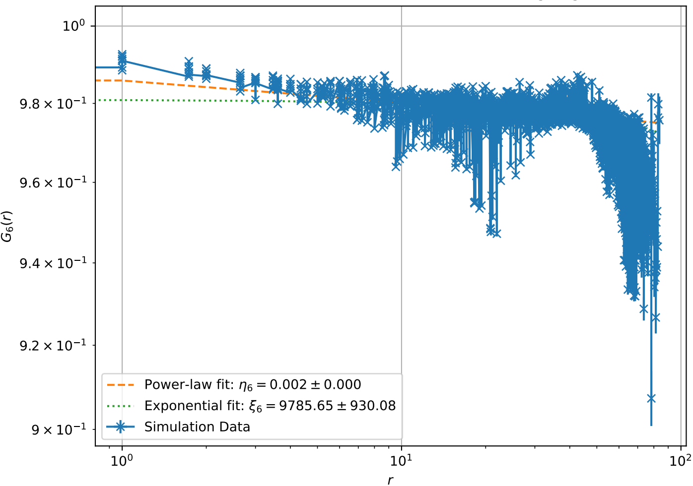
Correlation Function at T = 6.00e - 02 , L = 64 (Log-Log Scale)
