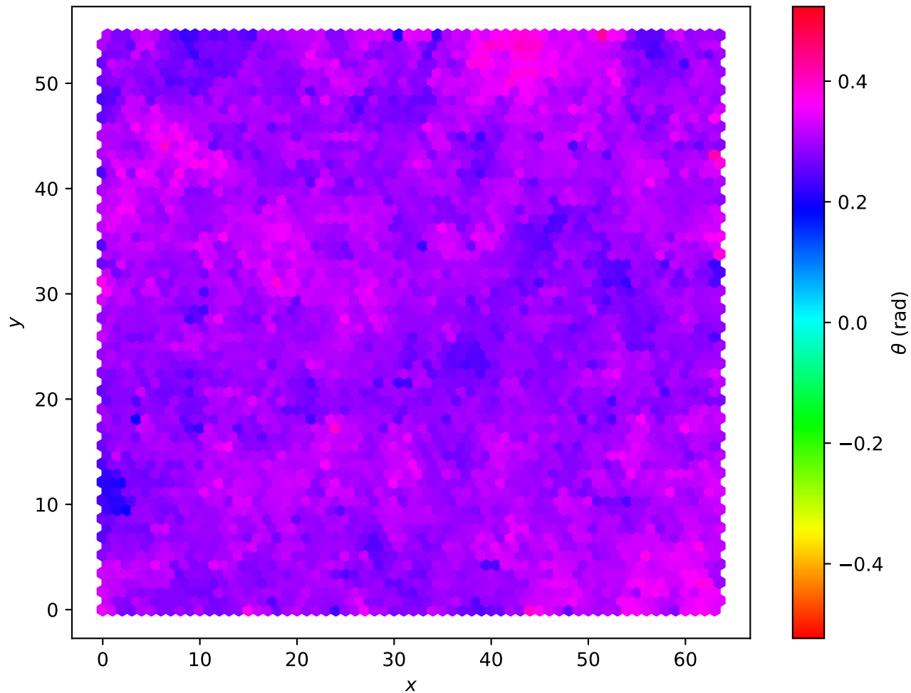
Hexagonal Lattice L=64 , T = 6.00e - 02
