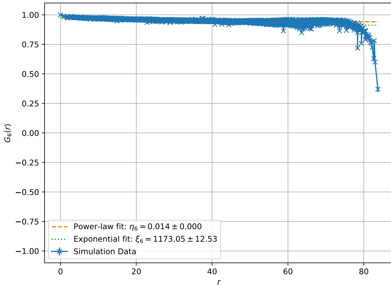
Correlation Function at T = 7.00e - 02 , L = 64
