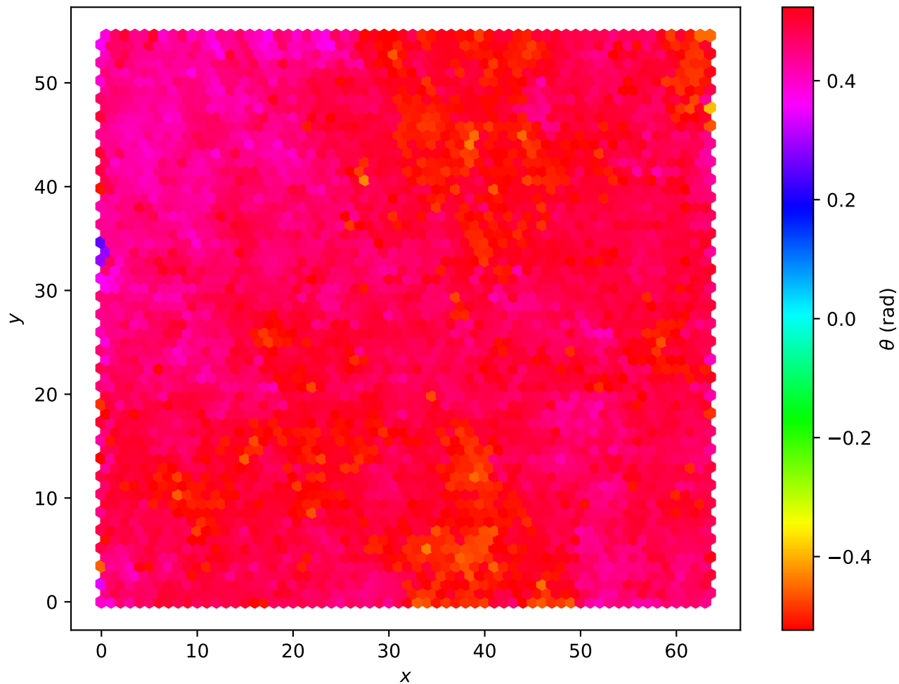
Hexagonal Lattice L=64 , T = 7.00e - 02
