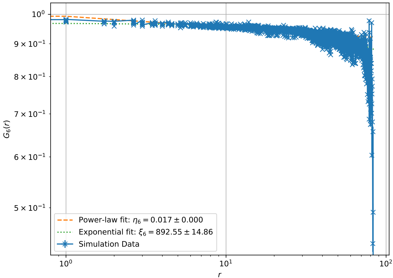
Correlation Function at T = 8.00e - 02 , L = 64 (Log-Log Scale)
