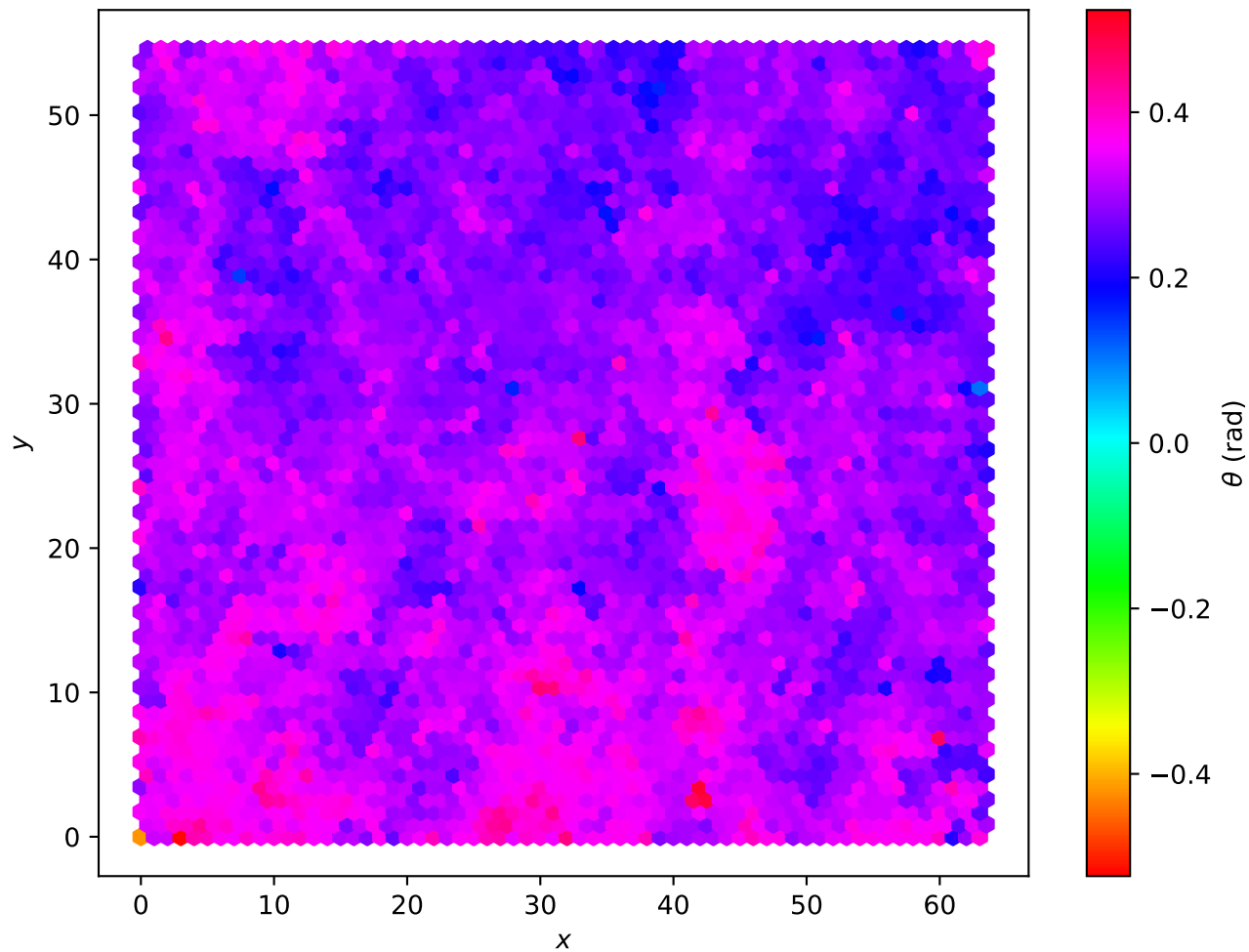
Hexagonal Lattice L=64 , T = 8.00e - 02
