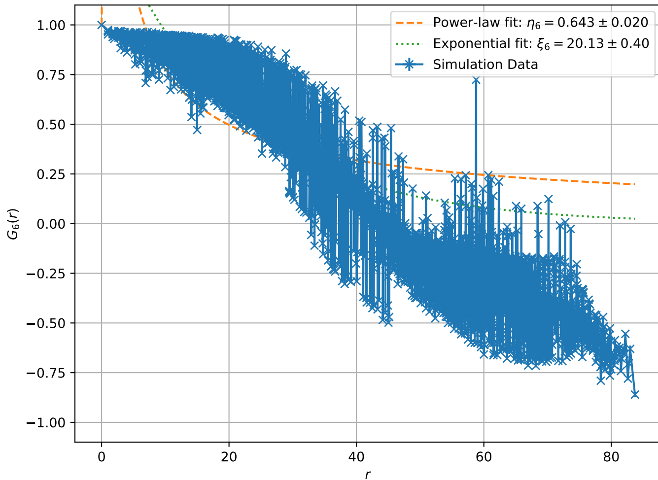
Correlation Function at T = 9.00e - 02 , L = 64
