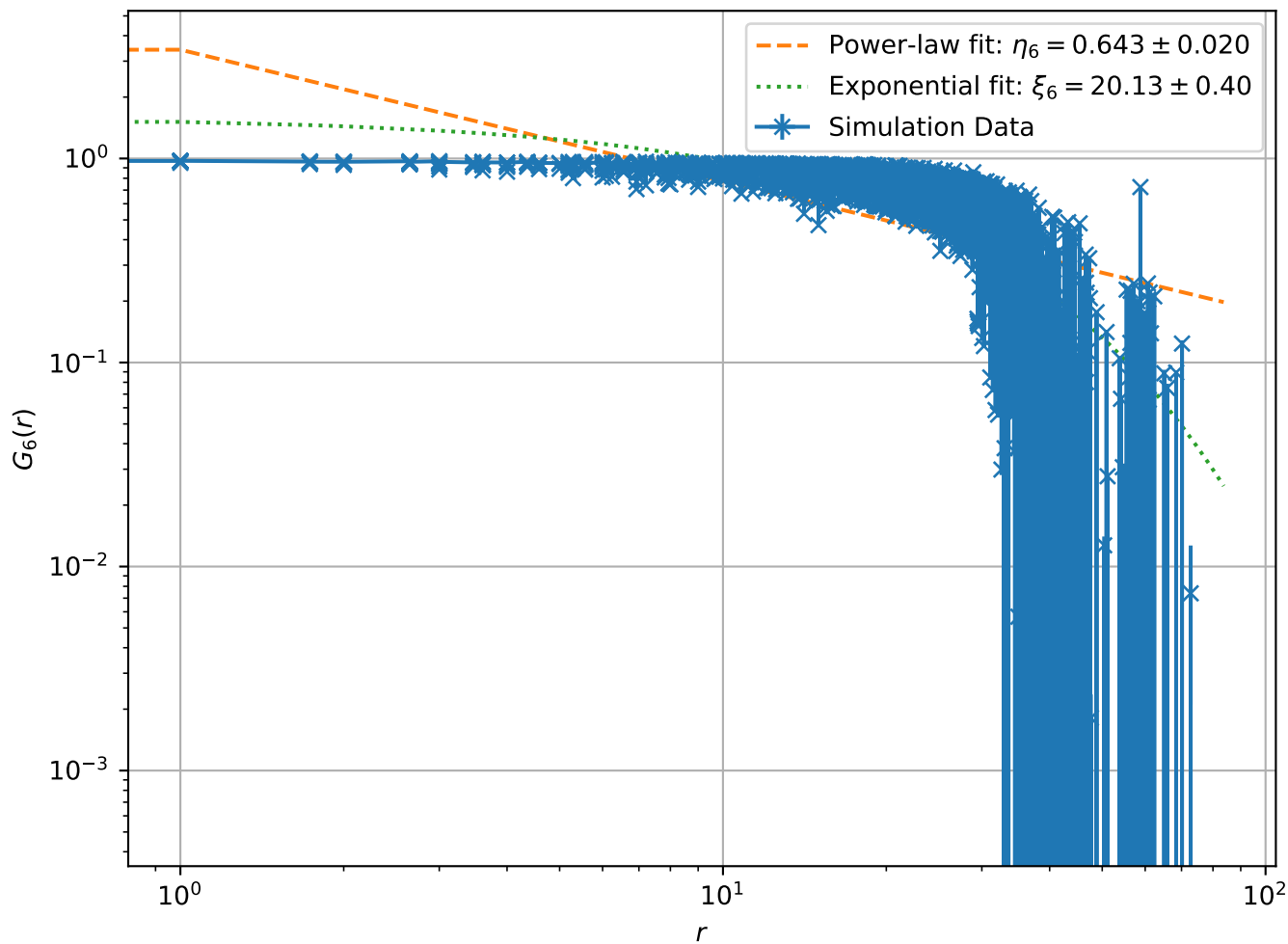
Correlation Function at T = 9.00e - 02 , L = 64 (Log-Log Scale)
