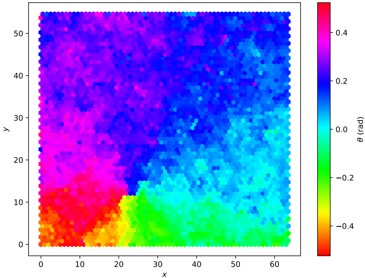
Hexagonal Lattice L=64 , T = 9.00e - 02
