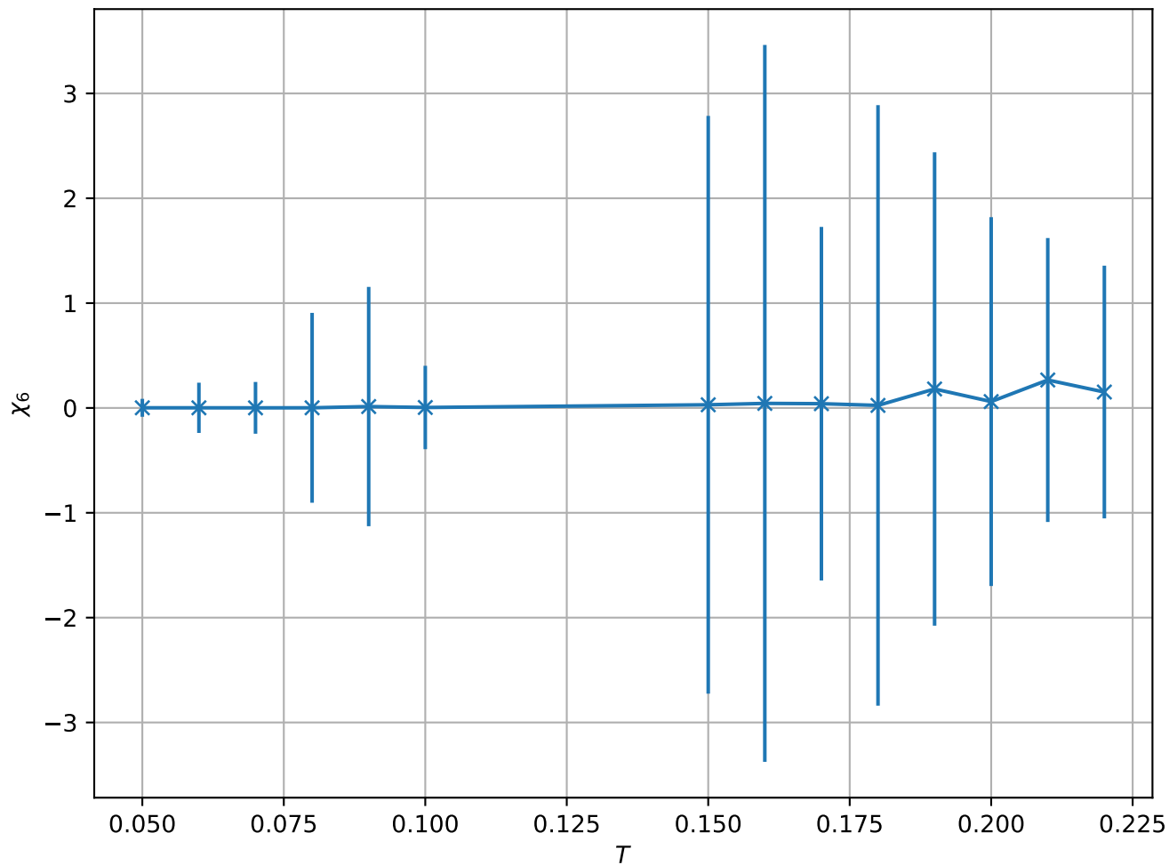
Susceptibility \chi_6 vs Temperature for L = 64
