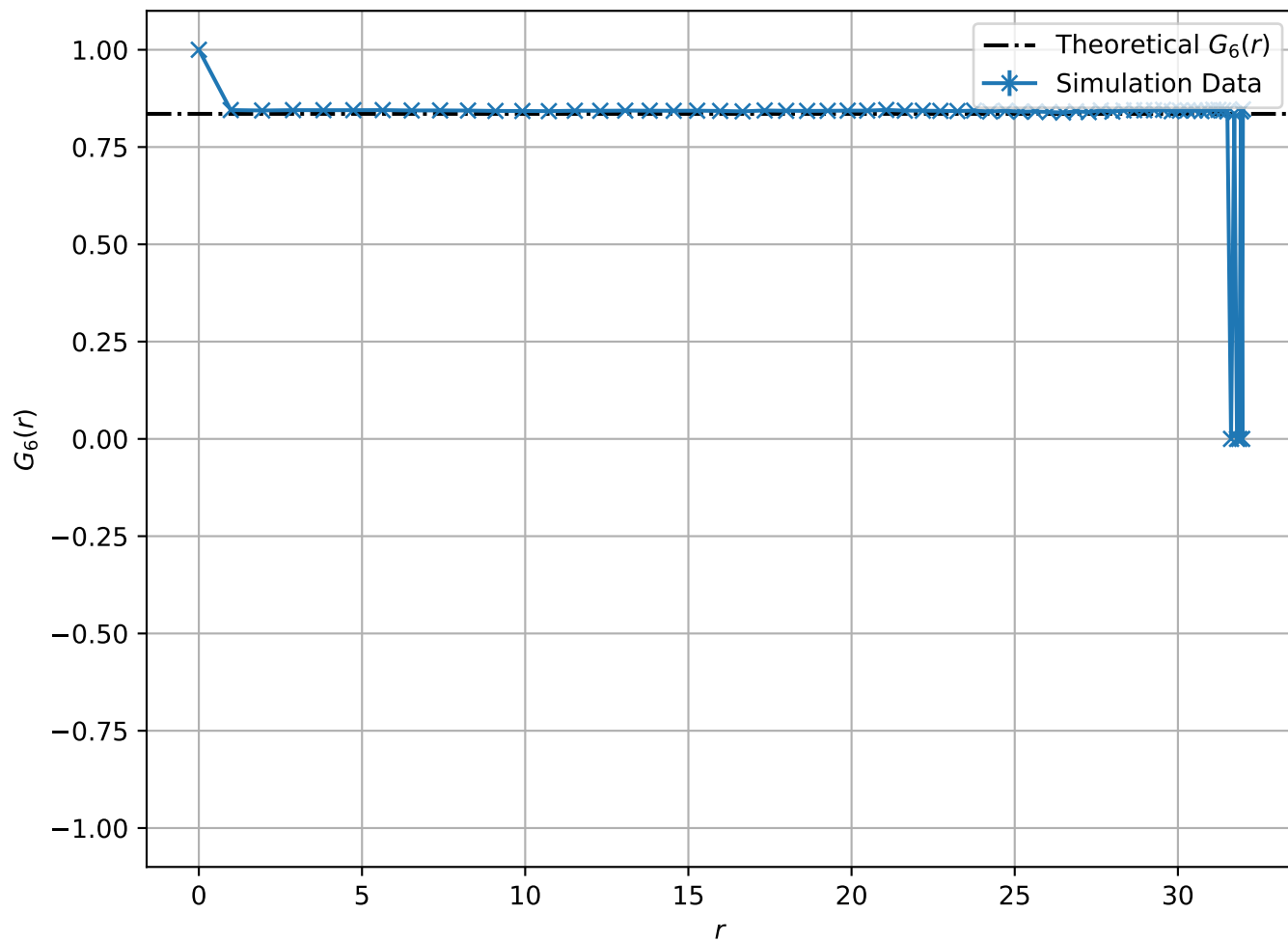
Correlation Function at T = 1.00e - 02 , L = 32
