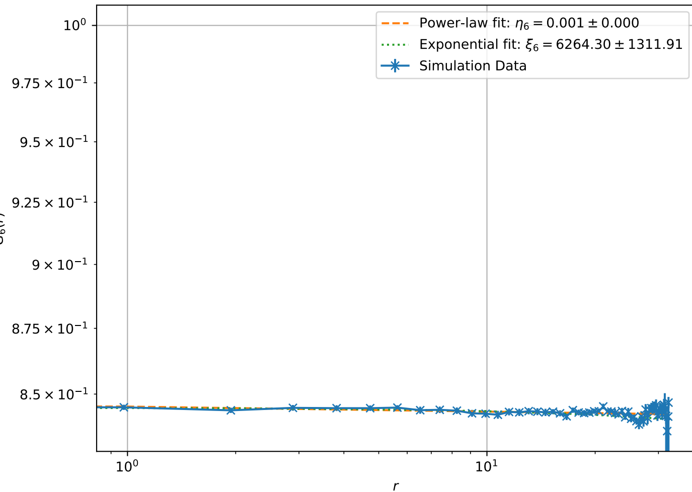
Correlation Function at T = 1.00e - 02 , L = 32 (Log-Log Scale)
