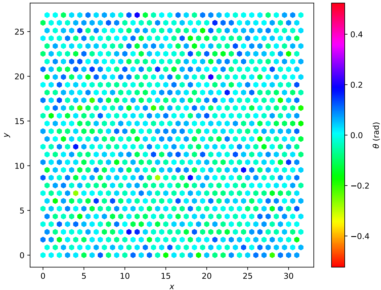
Hexagonal Lattice L=32 , T = 1.00e - 02
