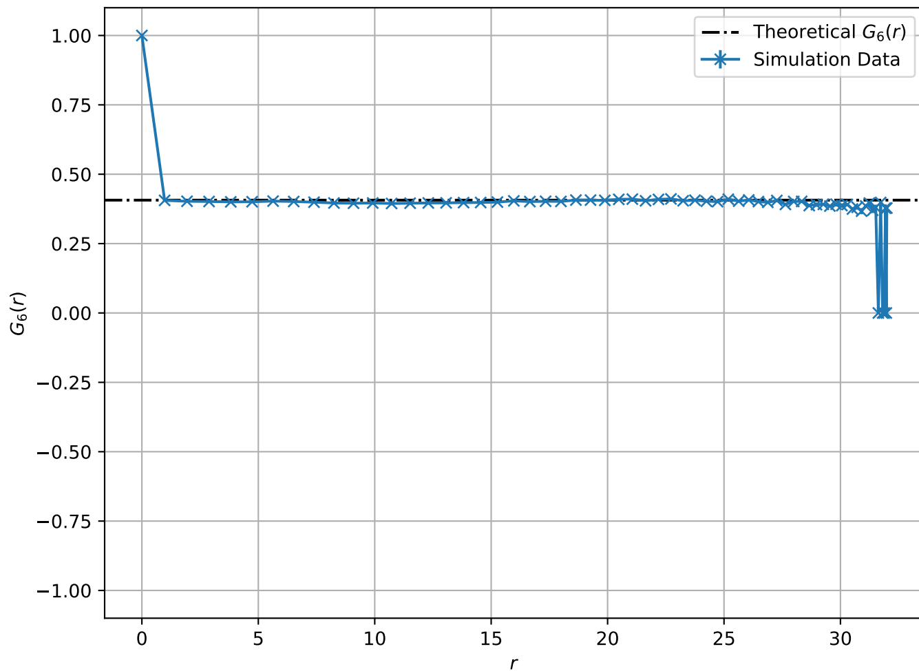
Correlation Function at T = 5.00e - 02 , L = 32
