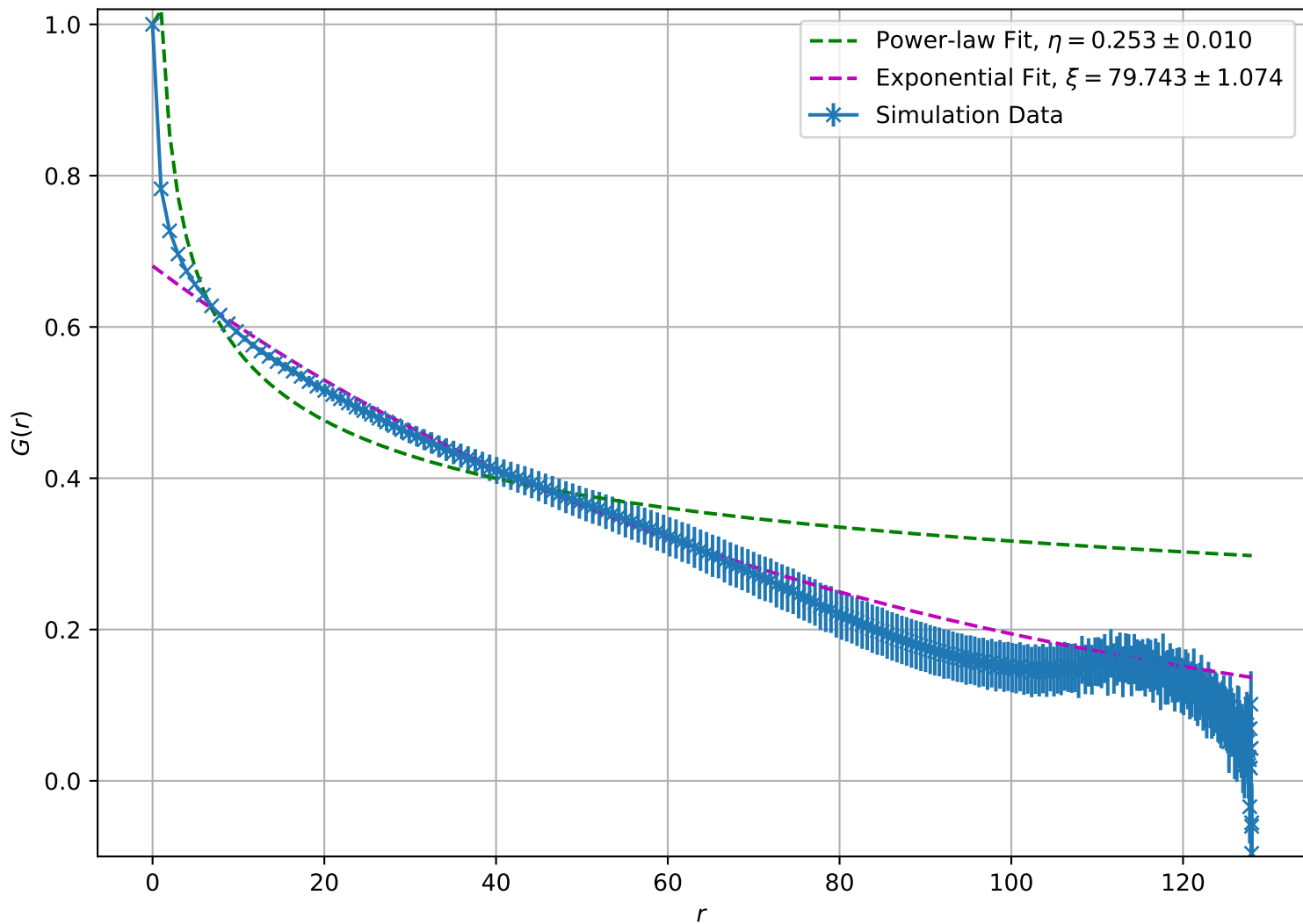
Correlation Function at T = 1.00\text{e} + 00 , L = 128
