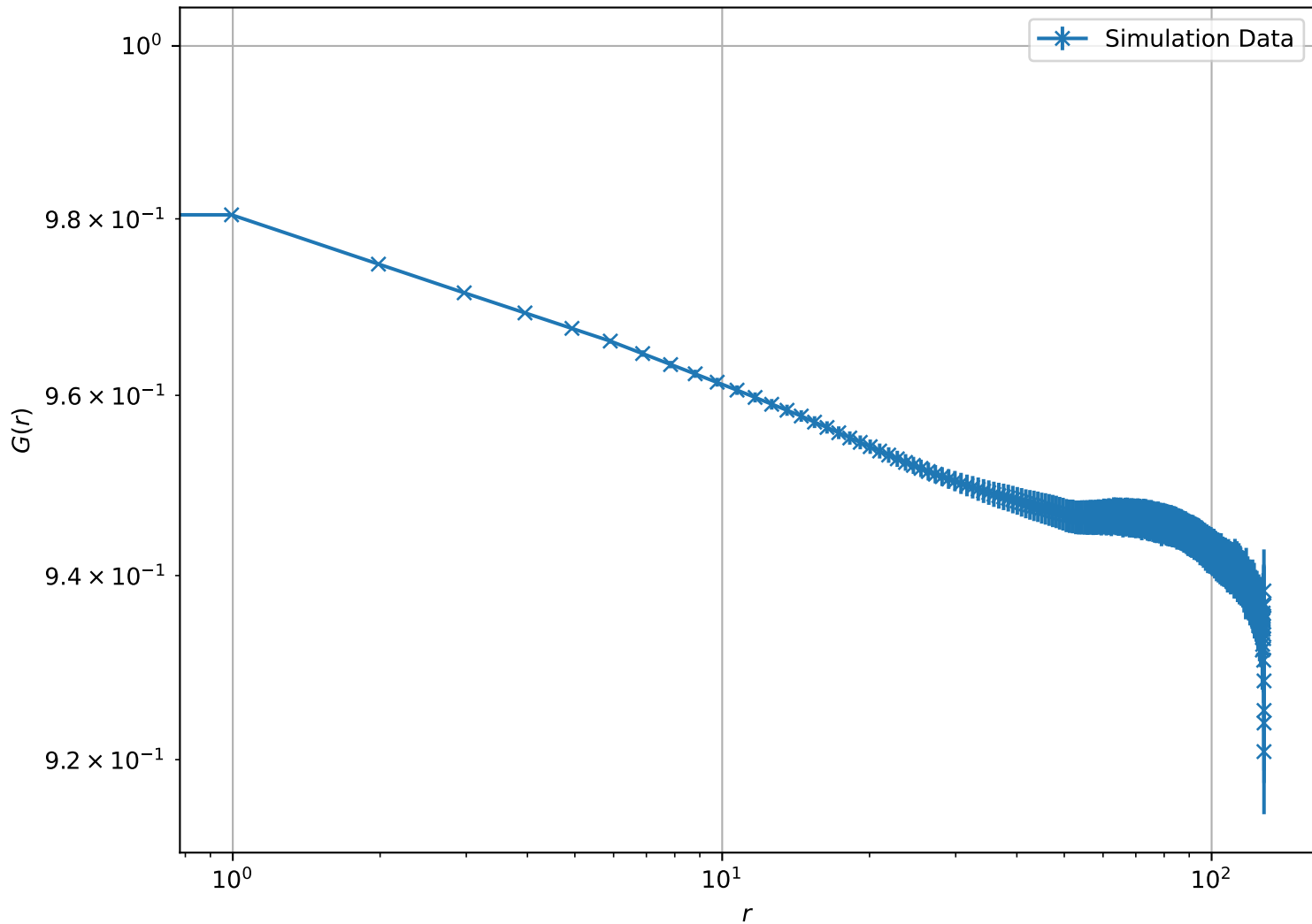
Correlation Function at T = 1.00e - 01 , L = 128 (Log-Log Scale)
