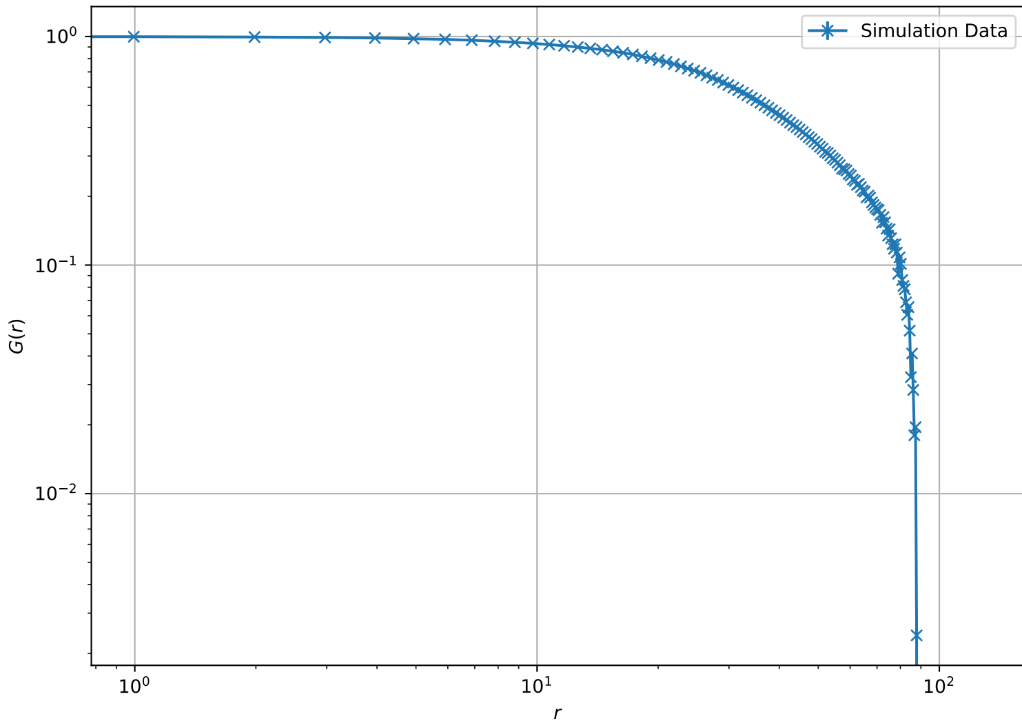
Correlation Function at T = 1.00\text{e} - 05 , L = 128 (Log-Log Scale)
