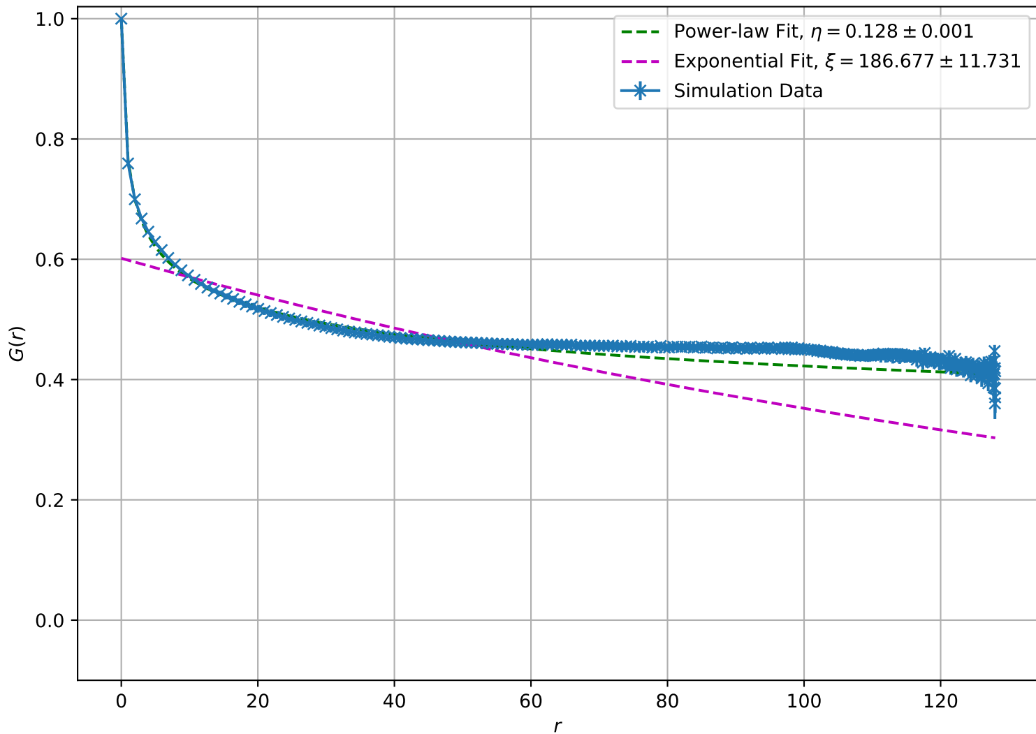
Correlation Function at T = 1.10e + 00 , L = 128
