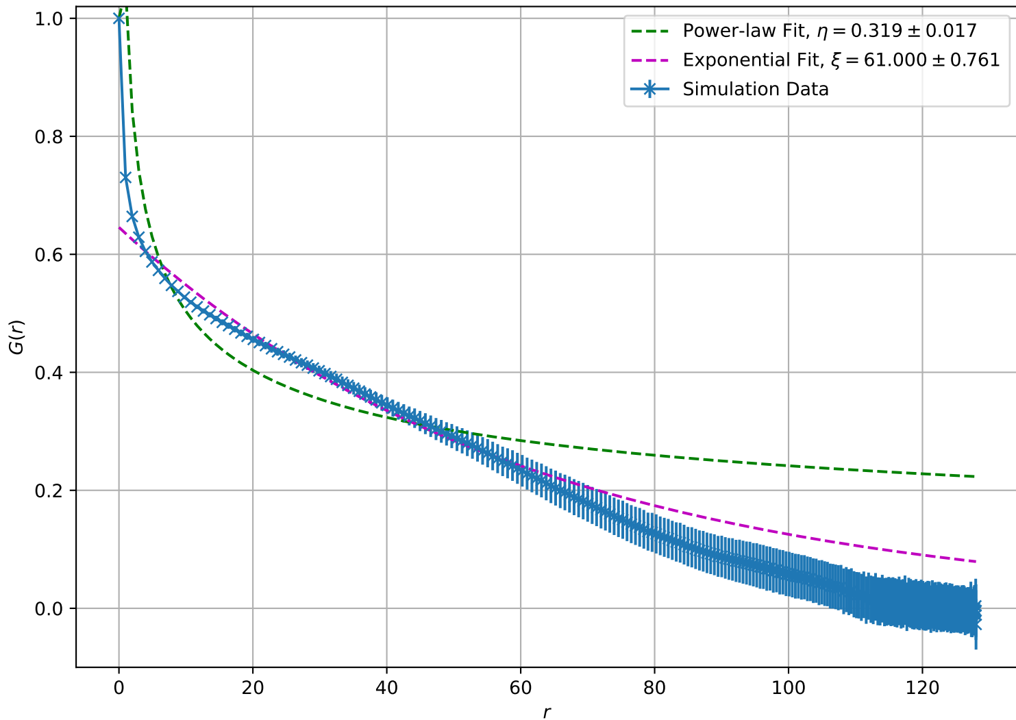
Correlation Function at T = 1.20\text{e} + 00 , L = 128
