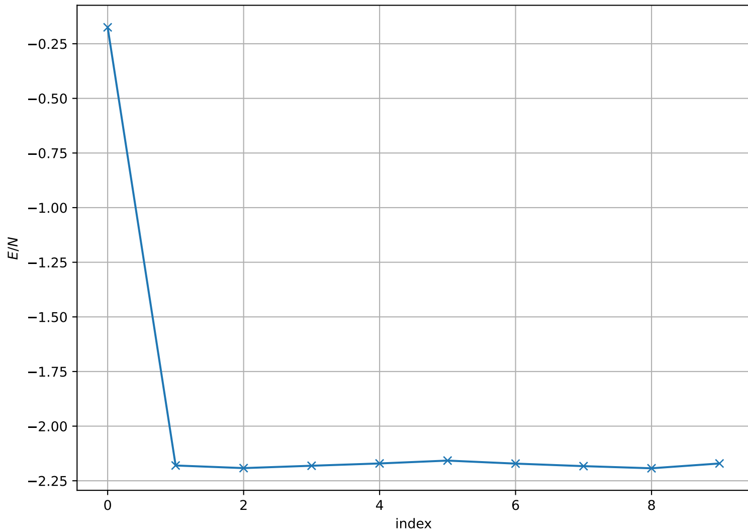
Energy per Site at T = 1.300e + 00 , L = 128
