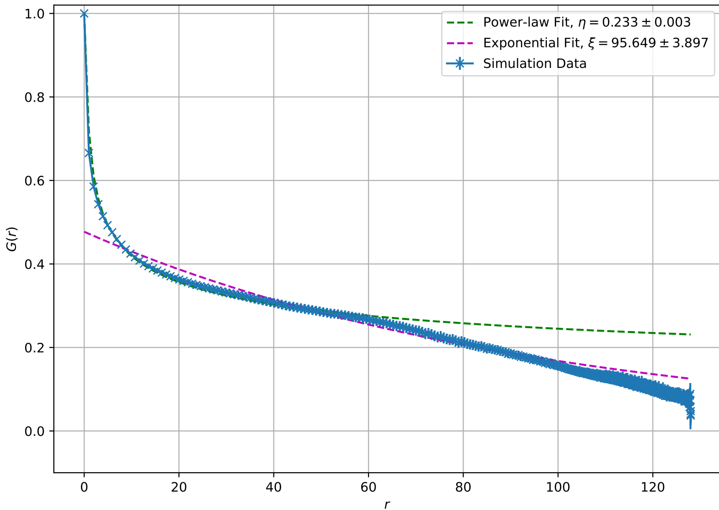
Correlation Function at T = 1.40e + 00 , L = 128
