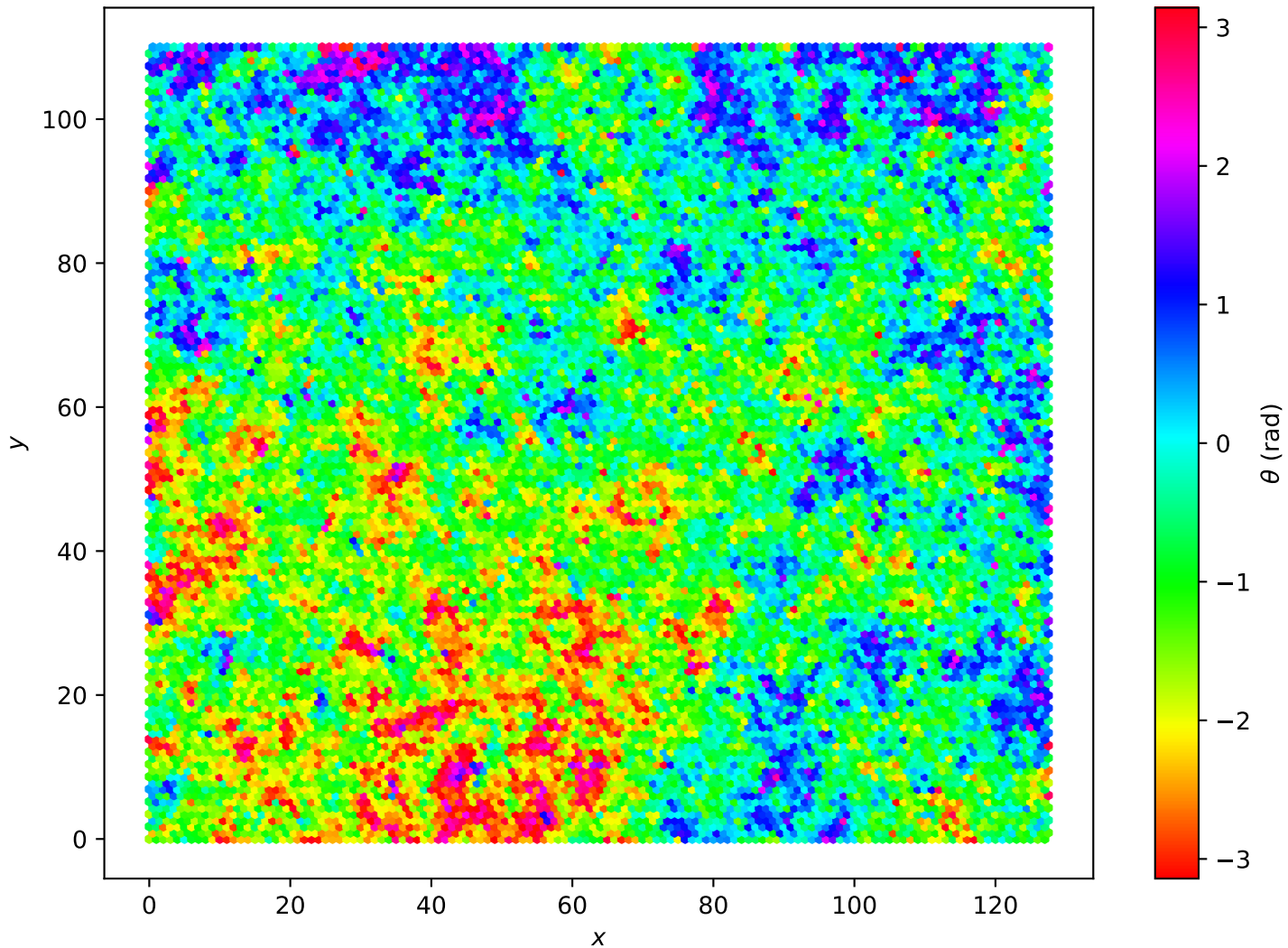
Hexagonal Lattice L=128 , T = 1.40e + 00
