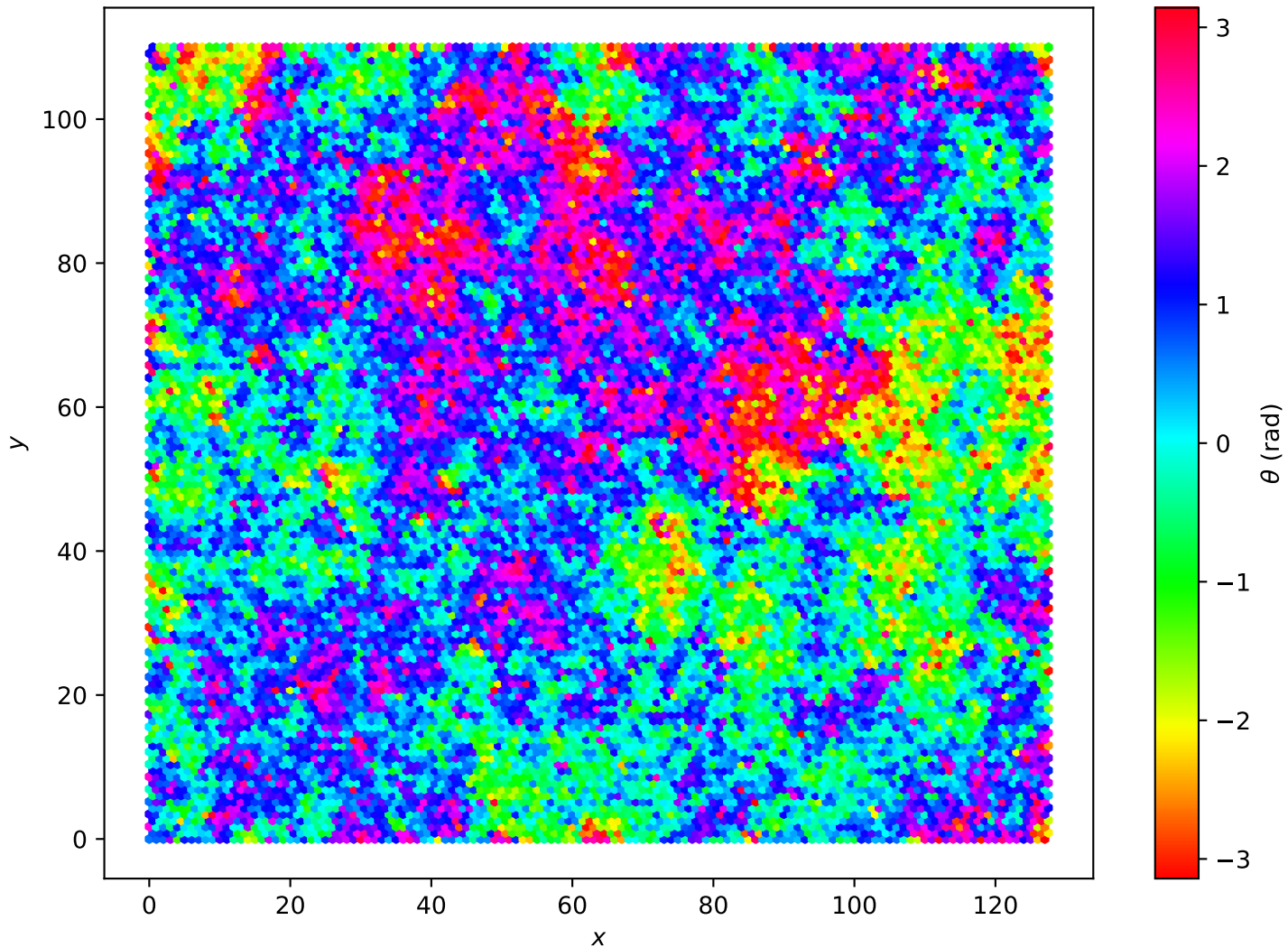
Hexagonal Lattice L=128 , T = 1.50e + 00
