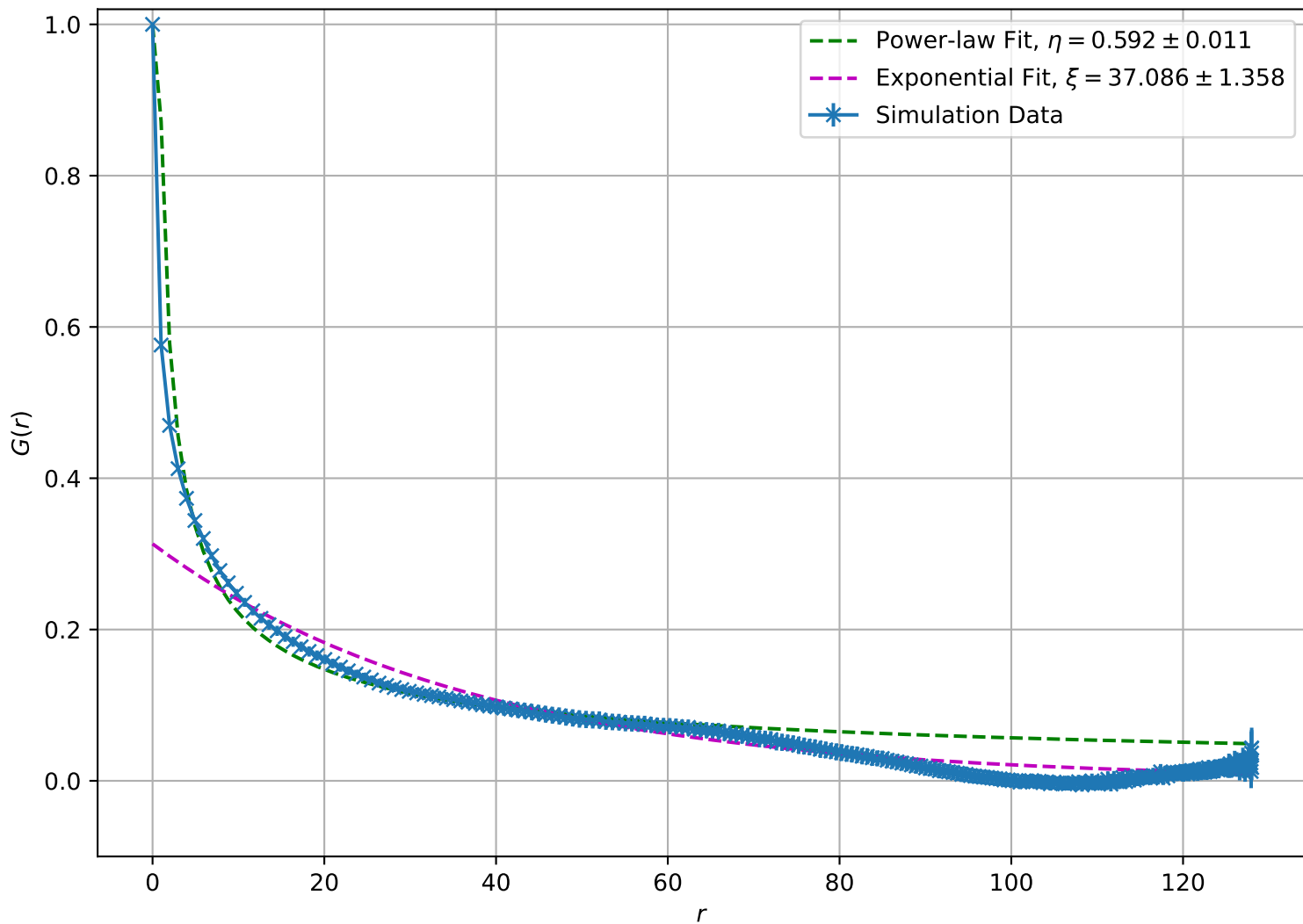
Correlation Function at T = 1.60\text{e} + 00 , L = 128
