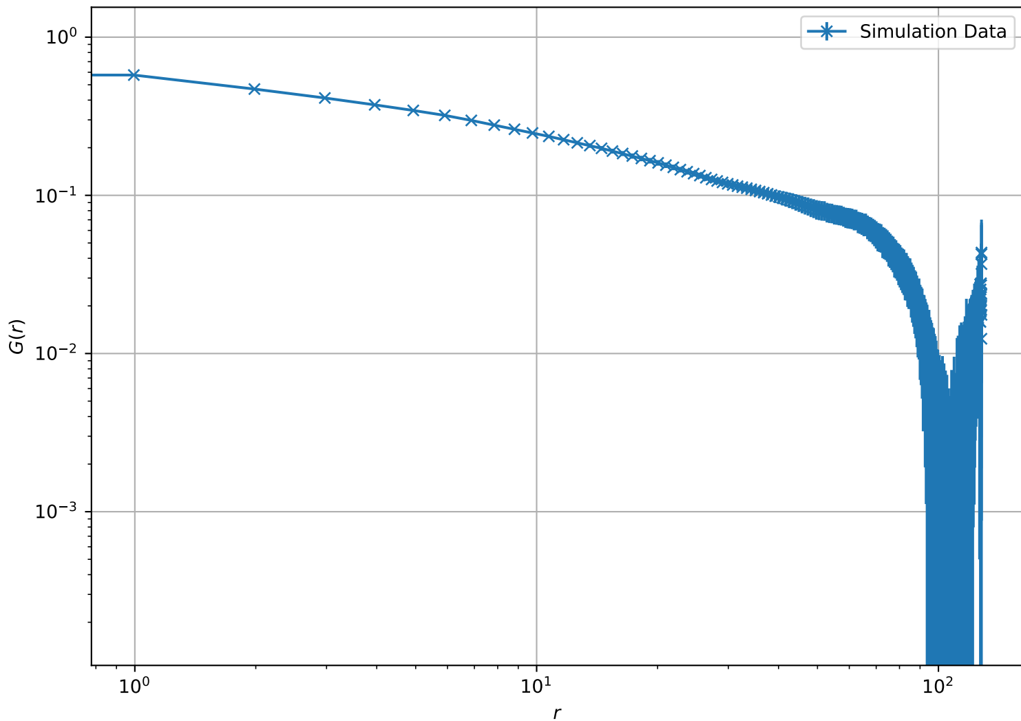
Correlation Function at T = 1.60e + 00 , L = 128 (Log-Log Scale)
