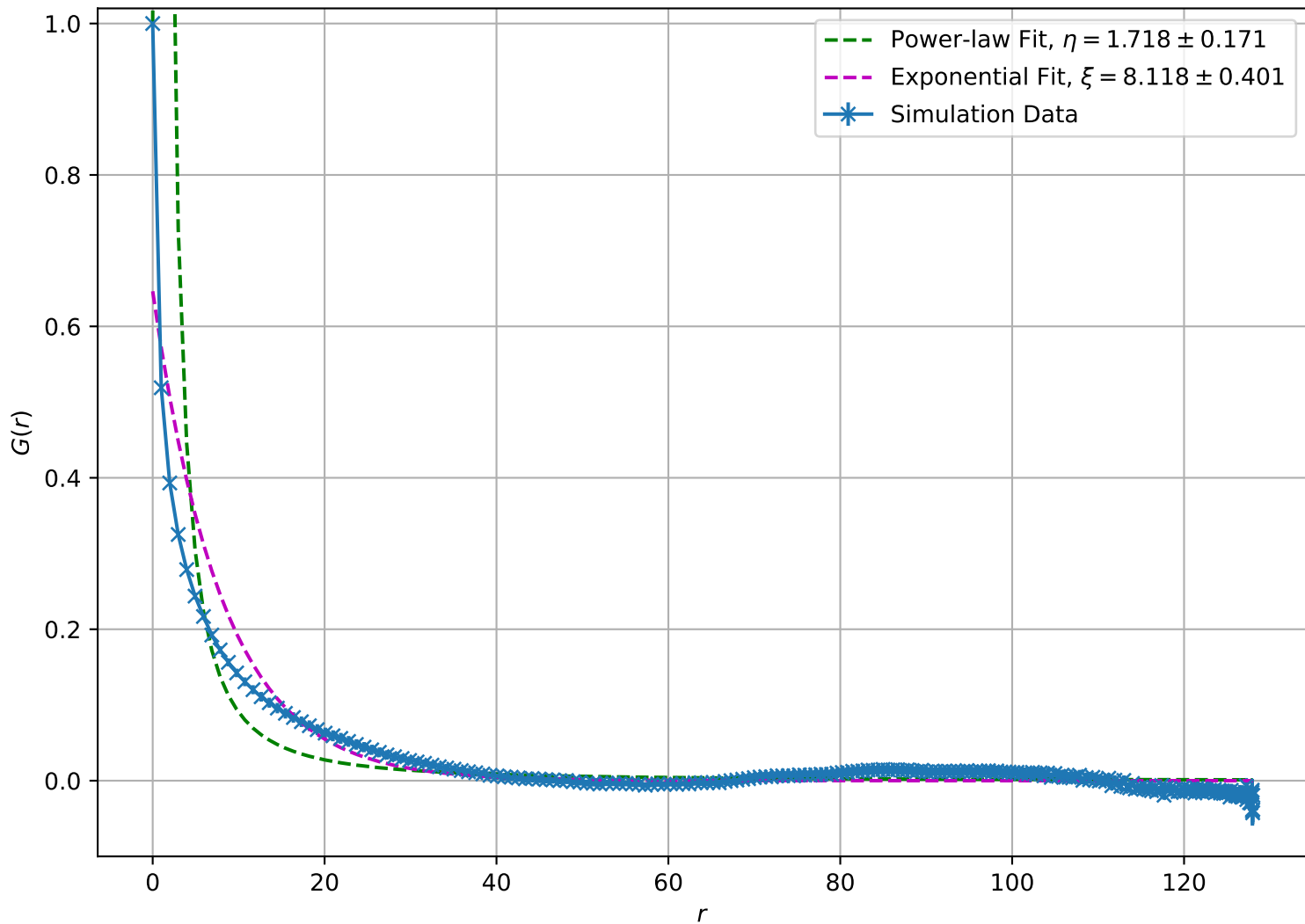
Correlation Function at T = 1.70e + 00 , L = 128
