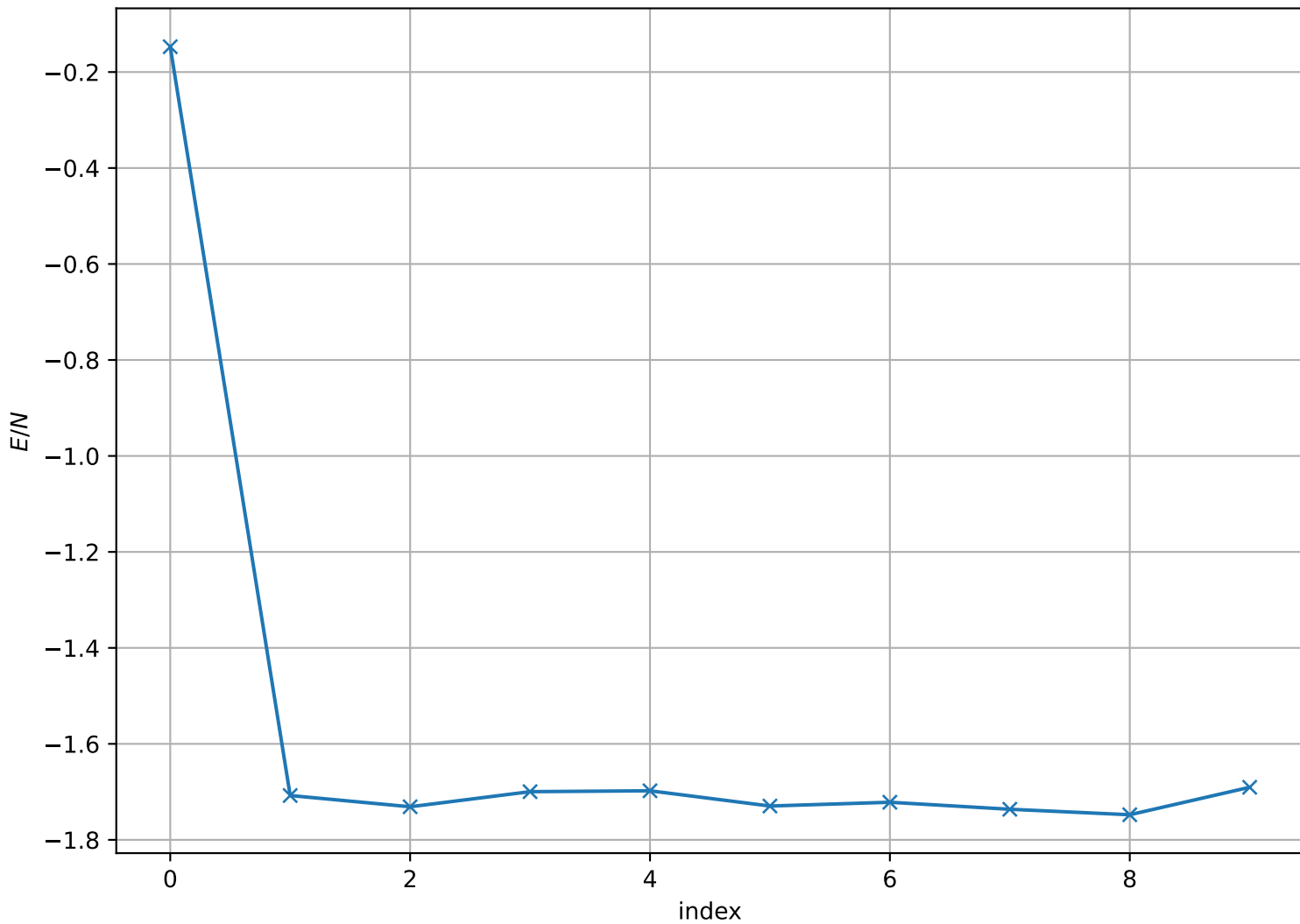
Energy per Site at T = 1.700e + 00 , L = 128
