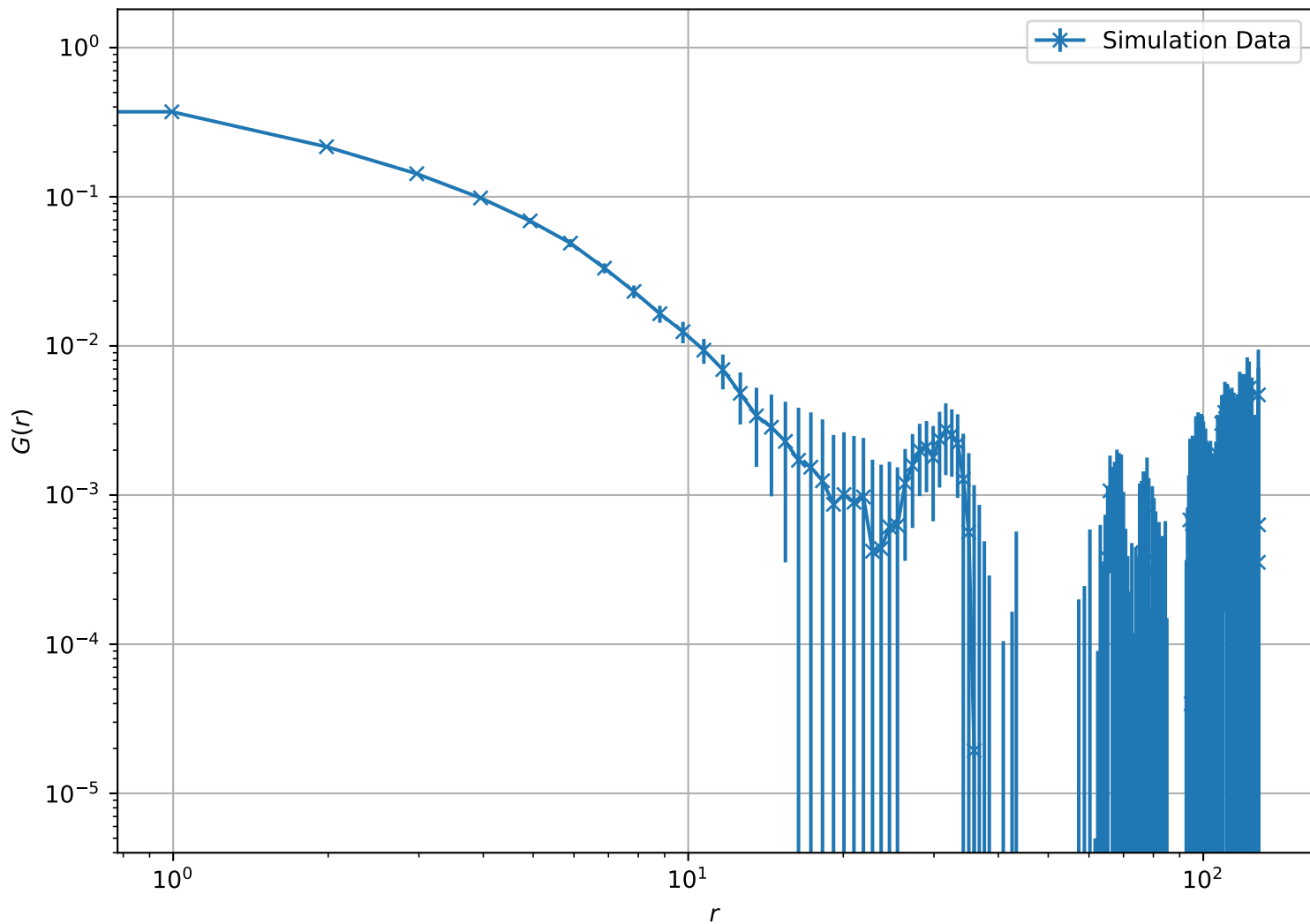
Correlation Function at T = 2.00e + 00 , L = 128 (Log-Log Scale)
