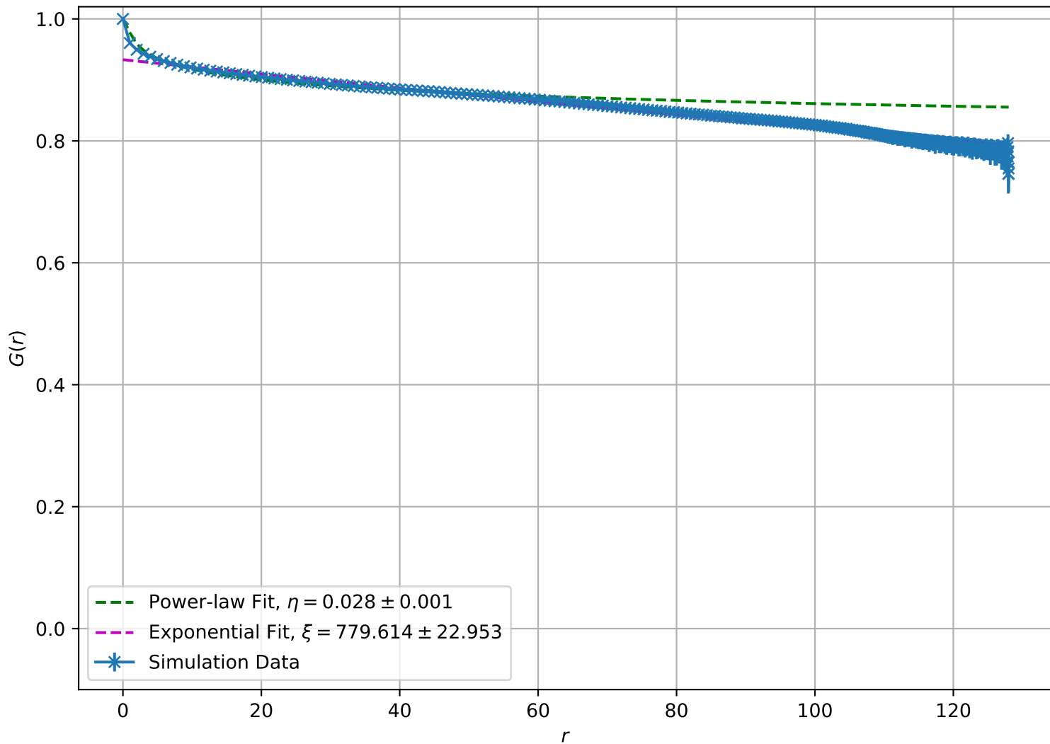
Correlation Function at T = 2.00e - 01 , L = 128
