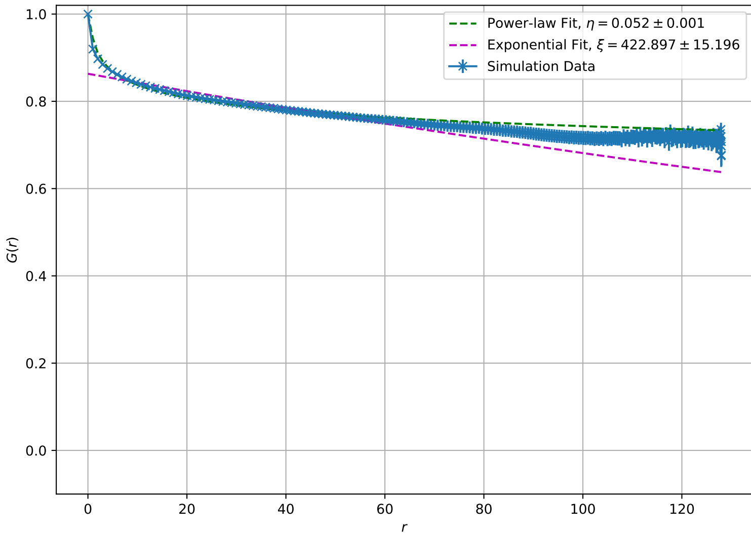
Correlation Function at T = 4.00e - 01 , L = 128
