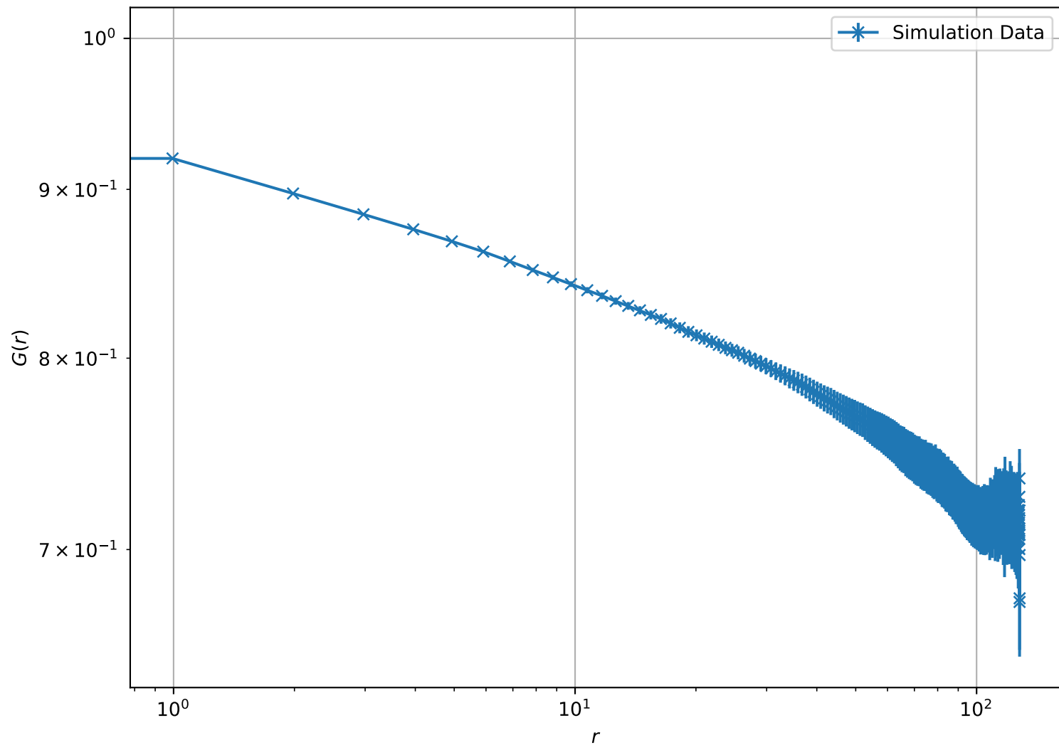
Correlation Function at T = 4.00e - 01 , L = 128 (Log-Log Scale)
