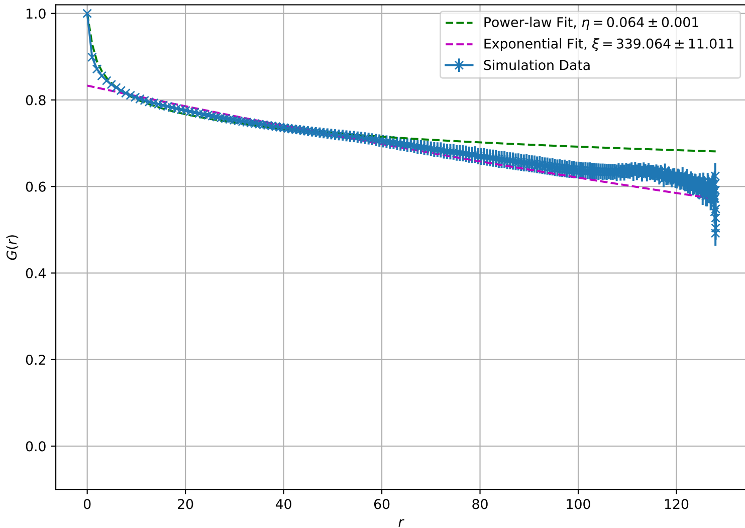
Correlation Function at T = 5.00e - 01 , L = 128
