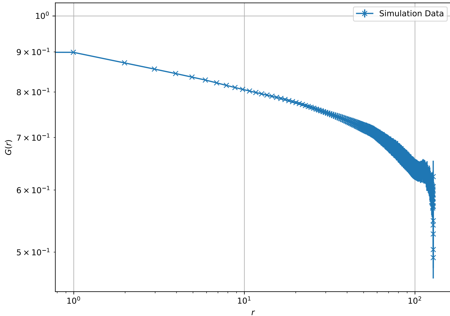
Correlation Function at T = 5.00e - 01 , L = 128 (Log-Log Scale)
