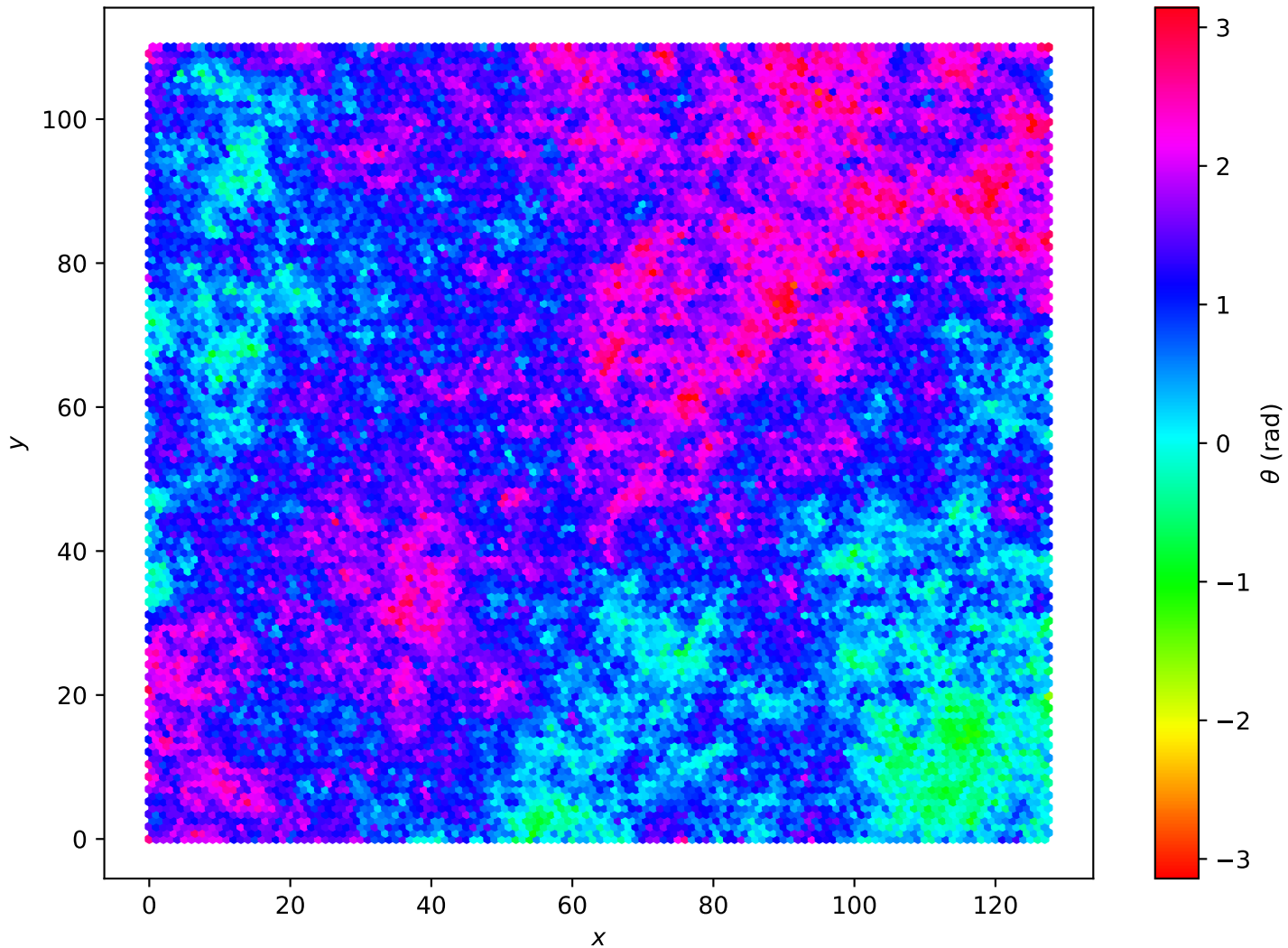
Hexagonal Lattice L=128 , T = 5.00e - 01
