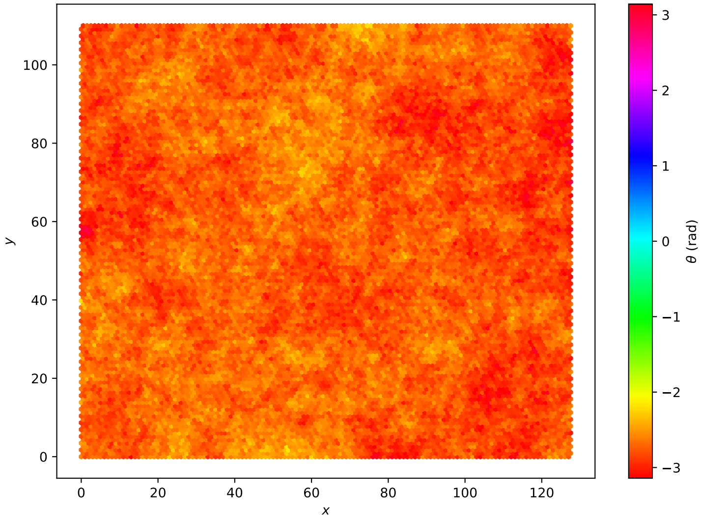
Hexagonal Lattice L=128 , T = 5.00e - 02
